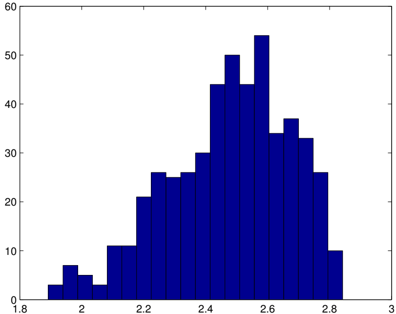
FIGURE 1. Distribution of the final time of controllability for N = 5 and for initial consensus parameters randomly generated 500 times.
