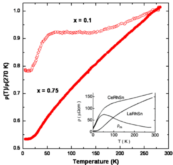
Fig. 8 (color online). Temperature dependence of the reduced electrical resistivity of \text{Ce}(\text{Rh}_{1-x}\text{Ru}_x)\text{Sn} with x=0.1 and 0.75 . The inset presents the temperature dependence of the electrical resistivity of \text{CeRhSn} and \text{LaRhSn} and also the magnetic resistivity \rho_m of \text{CeRhSn} [34].
