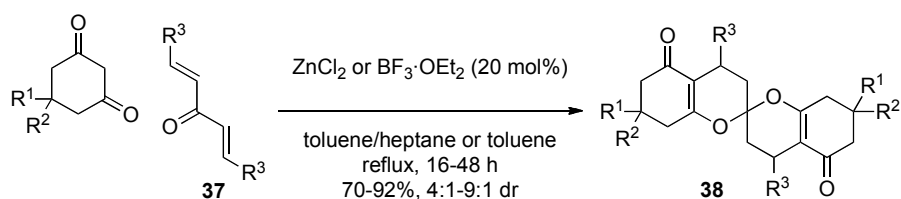
Scheme 11
