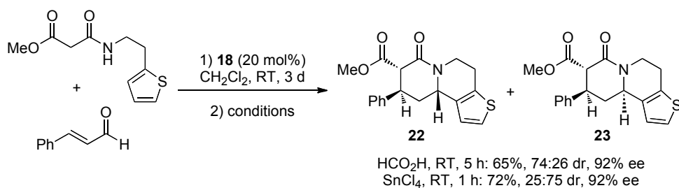
Scheme 7
