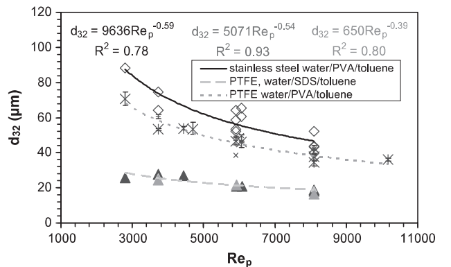
Fig. 22. Mean Sauter diameter versus the pulsation Reynolds number for the three systems at \Phi = 25\% and H = 1 m.
