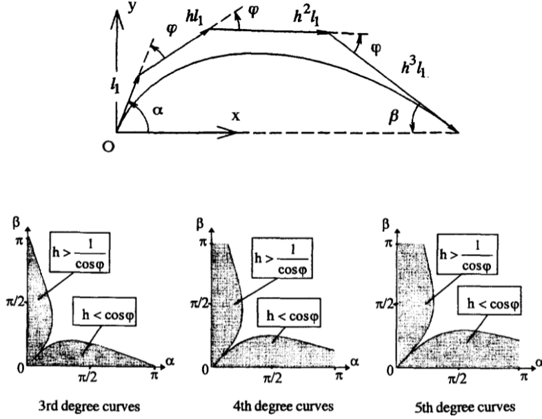
Fig. 2. Regions for a monotonic curvature variation.
