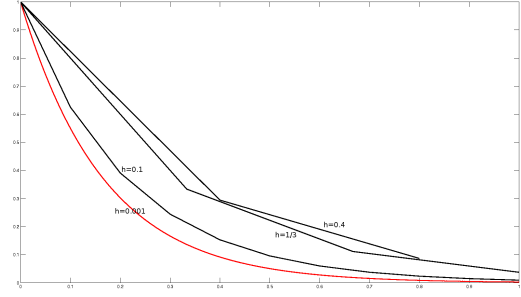
Fig. 3. An application of Implicit Euler scheme for the test-equation y' = -6y with the same values of the time step as in figure 2.
