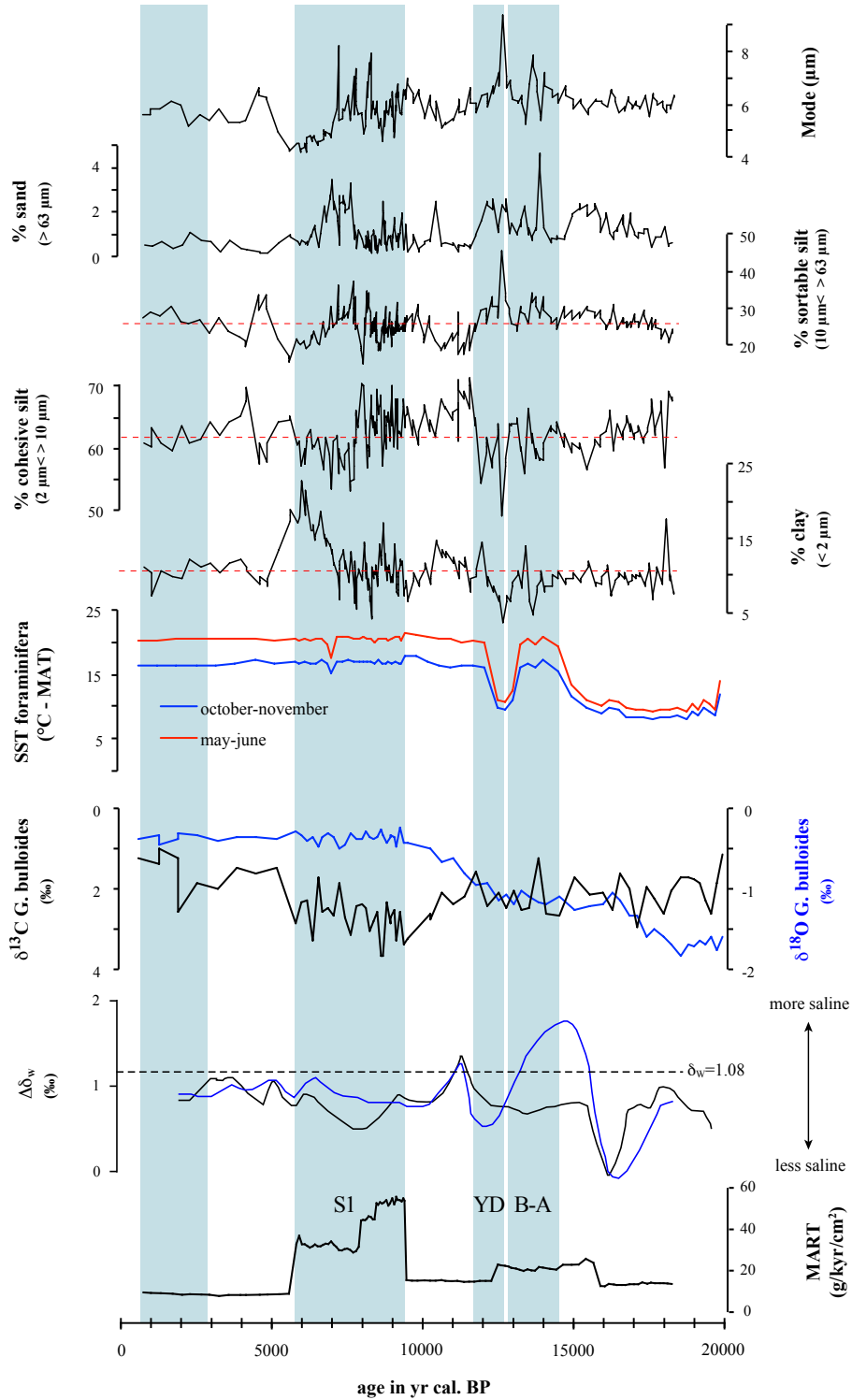
Fig. 3. Grain size analysis of core MD04-2797: main mode ( \mu\text{m} ), % of sand ( > 63 \mu\text{m} ), % of sortable silt ( 10 < > 63 \mu\text{m} ), % of cohesive silt ( 2 < > 10 \mu\text{m} ) and % of clay ( < 2 \mu\text{m} ). MART ( \text{g kyr}^{-1}\text{cm}^{-2} ) from Fig. 2. Sea surface temperatures (SST) for May–June and October–November based on foraminifera association (Essallami et al., 2007), \delta^{18}\text{O} (‰) and \delta^{13}\text{C} from planktonic foraminifera G. bulloides (Essallami et al., 2007). \Delta\delta_w (‰) values are calculated using SSTs derived from MAT (blue) and alkenones (black) (Essallami et al., 2007). Mean analytical uncertainty is \pm 0/3 ‰.
