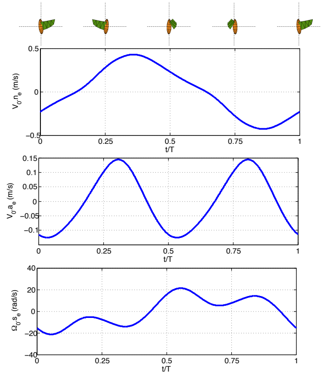
Fig. 7. The time evolution of the linear and angular speeds of B_0 in the sagittal plan of the robot for one stroke cycle.
