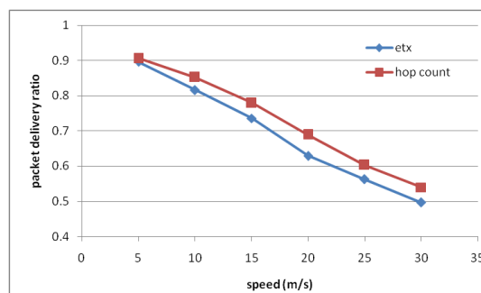
Figure 4.18 delivery ratio of ETX and hop count
