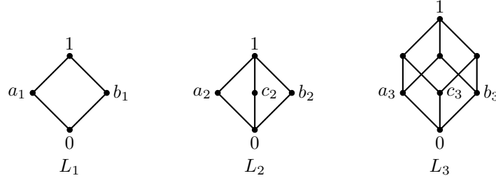
FIGURE 1. The lattices L_1 , L_2 and L_3 from Example 3.11.
