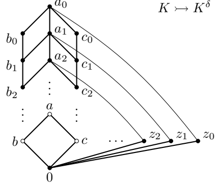
FIGURE 4. The lattice K , for which (J^\infty(K^\delta), \tau_c) is not spectral.
