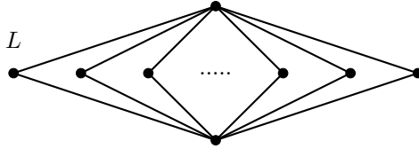
FIGURE 3. The lattice L , a countable antichain with top and bottom.
