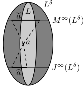
FIGURE 2. Topological spaces from the embedding of a lattice L into its canonical extension L^\delta .
