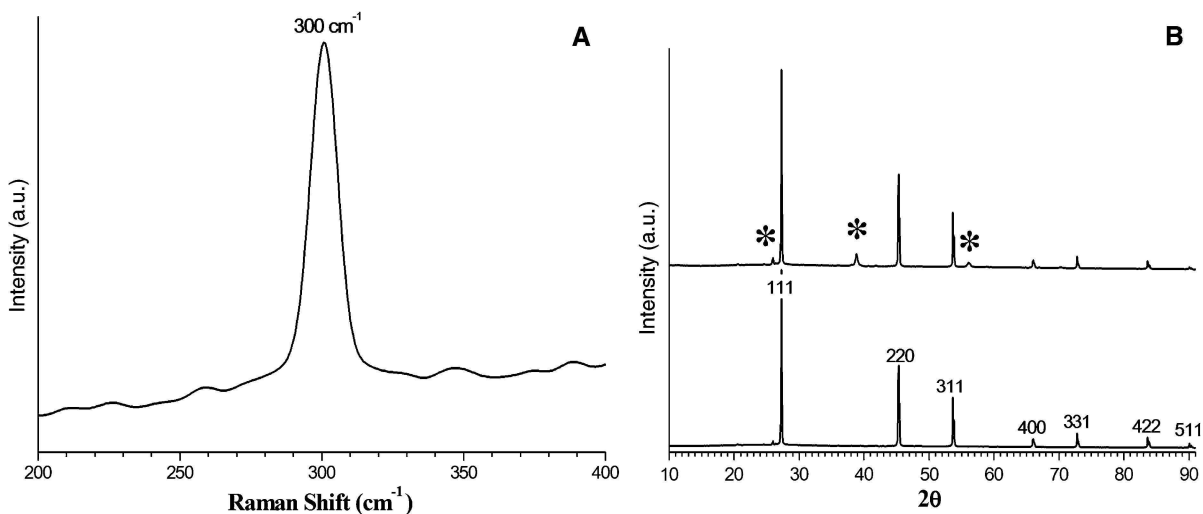
Fig. 6 Raman spectrum for a sample from route III with benzyl alcohol (a) and its XRD powder pattern indexed with cubic Ge (b)
