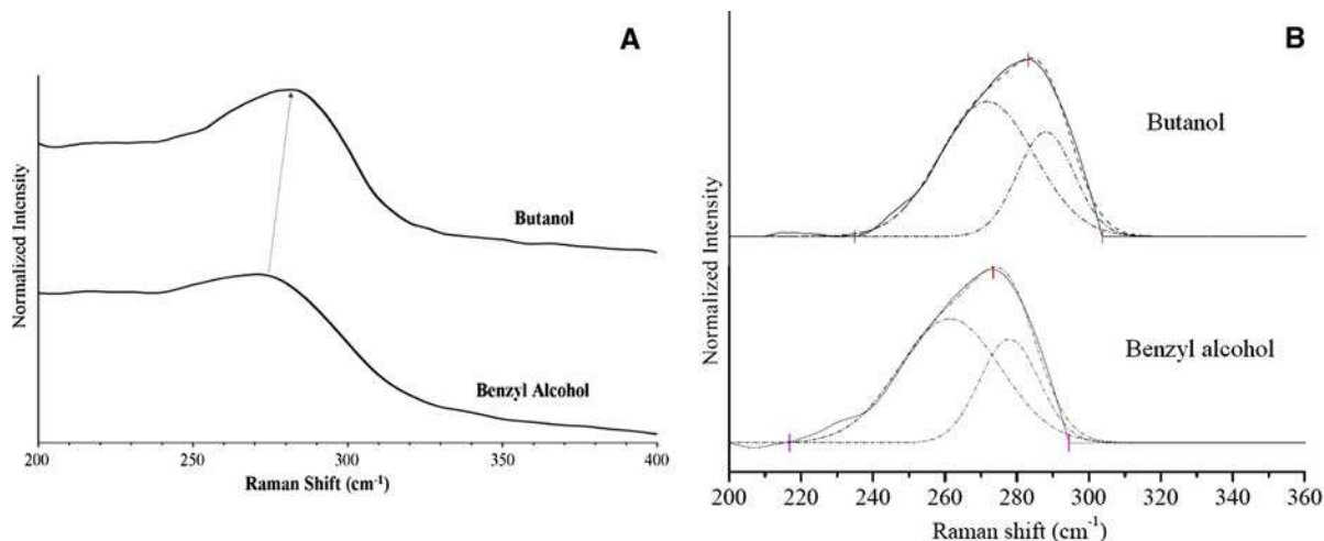
Fig.4 a Raman spectra of Ge nanopowders illustrating the increase in Raman shift (from benzyl alcohol to butanol). b Fitted spectra after background correction
