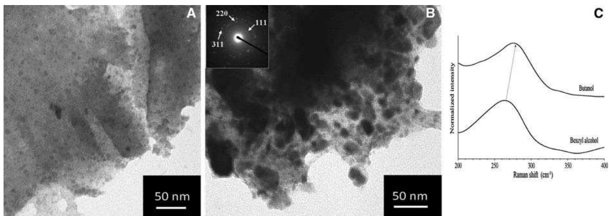
Fig. 5 TEM micrographs of Ge nanoparticles obtained from route II in benzyl alcohol (a) and butanol (b), Raman spectra of the corresponding materials (c)
