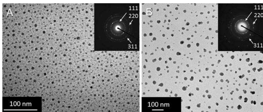
Fig. 3 TEM micrographs of crystalline Ge nanoparticles from route I using benzyl alcohol (a) and butanol (b) as oxidizing agent (insets SAED)
