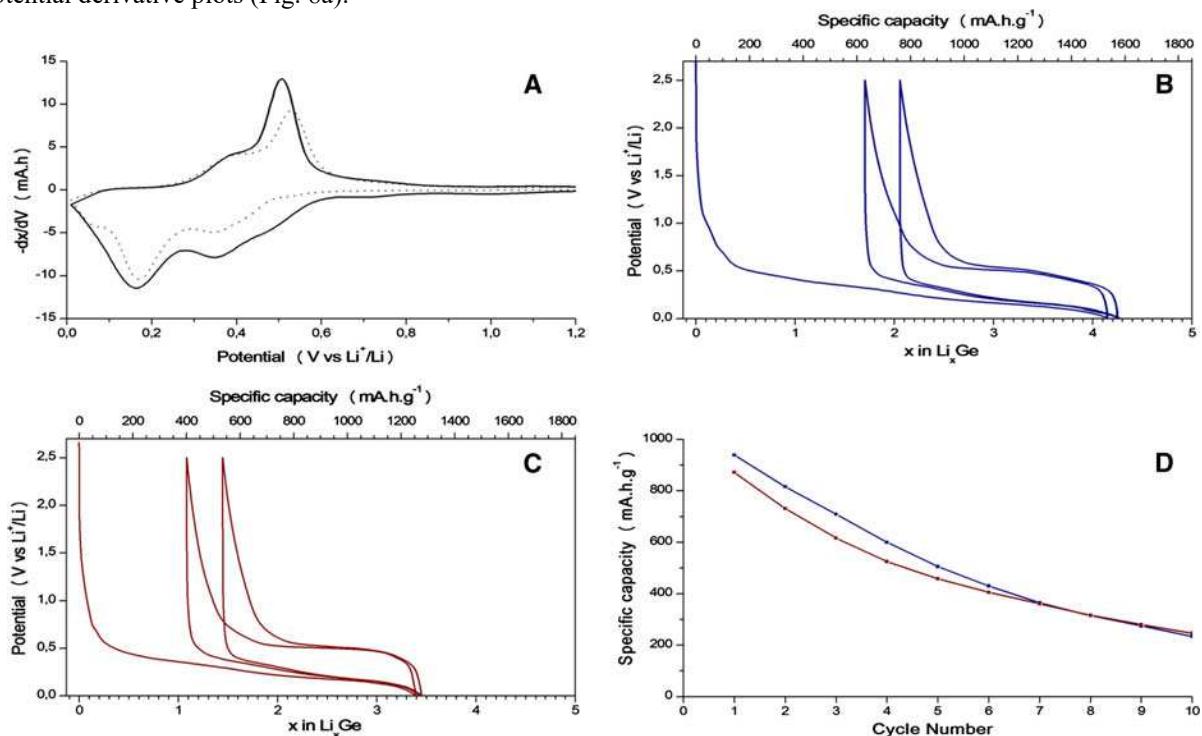
Fig. 8 Derivative plot dx/dV of small (plain line) and large (dotted line) particles (a), specific capacity for large (b) and small particles (c). d Comparative cycling performances
