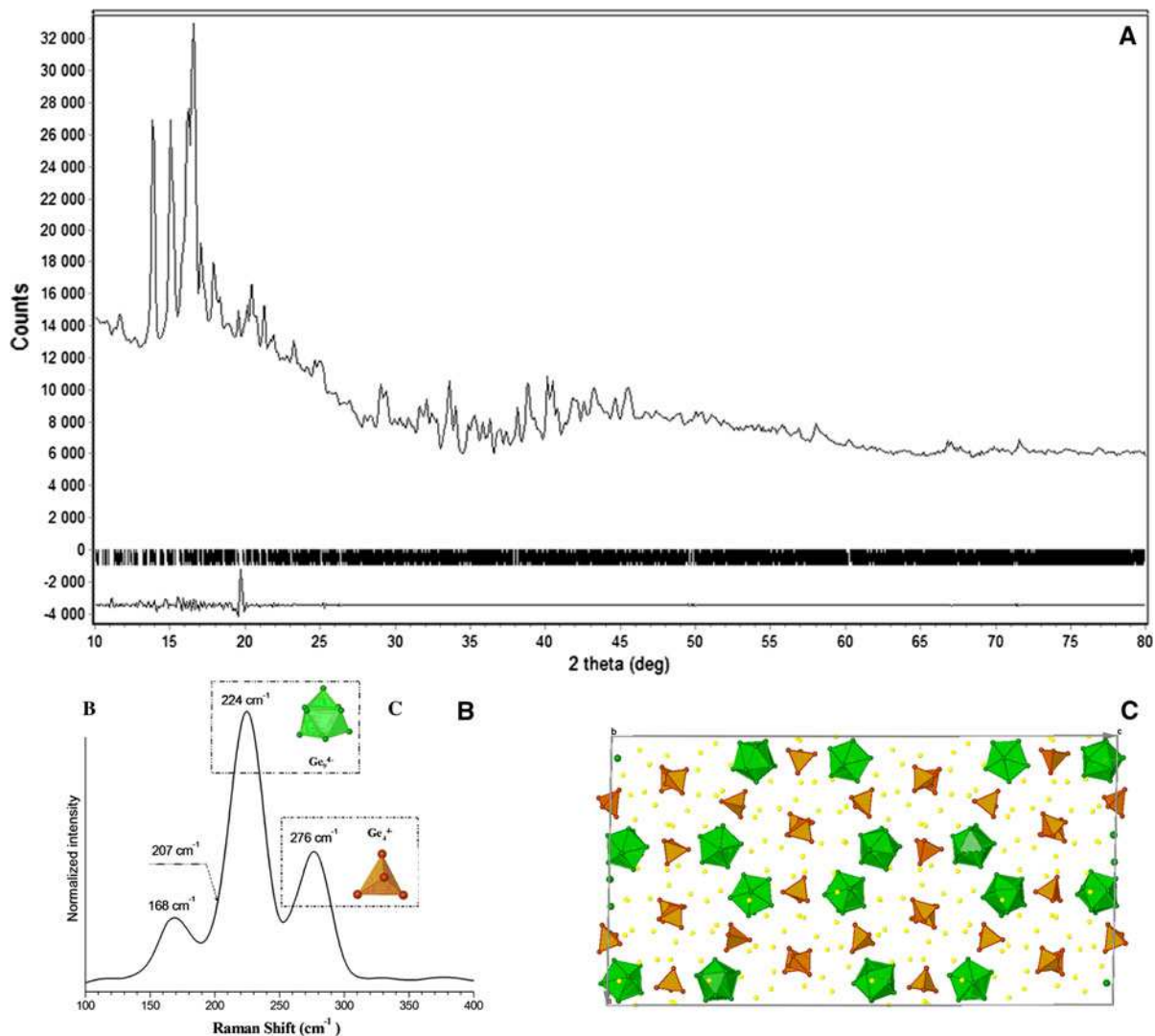
Fig. 2 X-ray diffractogram of \text{Na}_{12}\text{Ge}_{17} (a), Raman spectrum of \text{Na}_{12}\text{Ge}_{17} (b) and structure projection along b axis emphasizing the \text{Ge}_4^{4-} and \text{Ge}_9^{4-} anionic clusters (c)
