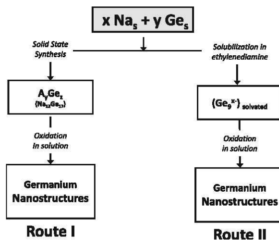
Fig. 1 Schematic representation of the synthetic routes I and II
