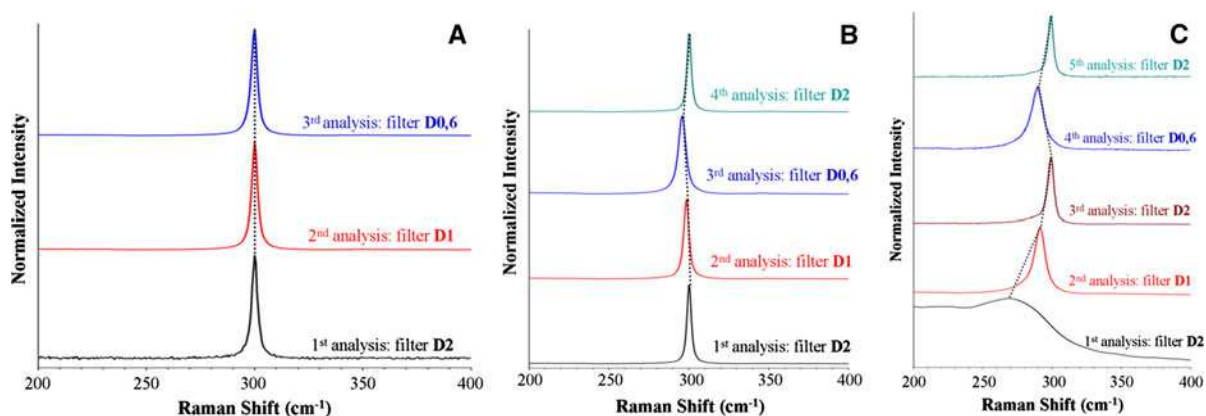
Fig. 7 Raman spectra under different irradiations for Ge wafers (a), Ge commercial powder (b), 5-nm Ge nanocrystals from route I (c)
