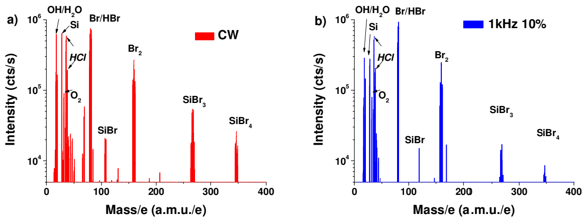
Figure 5. Mass spectra of neutrals during silicon etching in HBr/O 2 plasma a) in CW mode b) pulsed at 1kHz 10%
