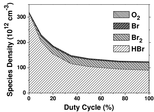
Figure 3. Species density measured by molecular beam mass spectrometry in a HBr/O 2 plasma pulsed at 1kHz. A duty cycle of 0% corresponds to the gas (no plasma struck) while a duty cycle of 100% correspond to a CW plasma
