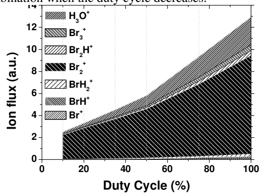
Figure 4. Ion flux composition determined by mass spectrometry in HBr/O 2 plasma pulsed at 1kHz. A duty cycle of 100% corresponds to the CW mode.
