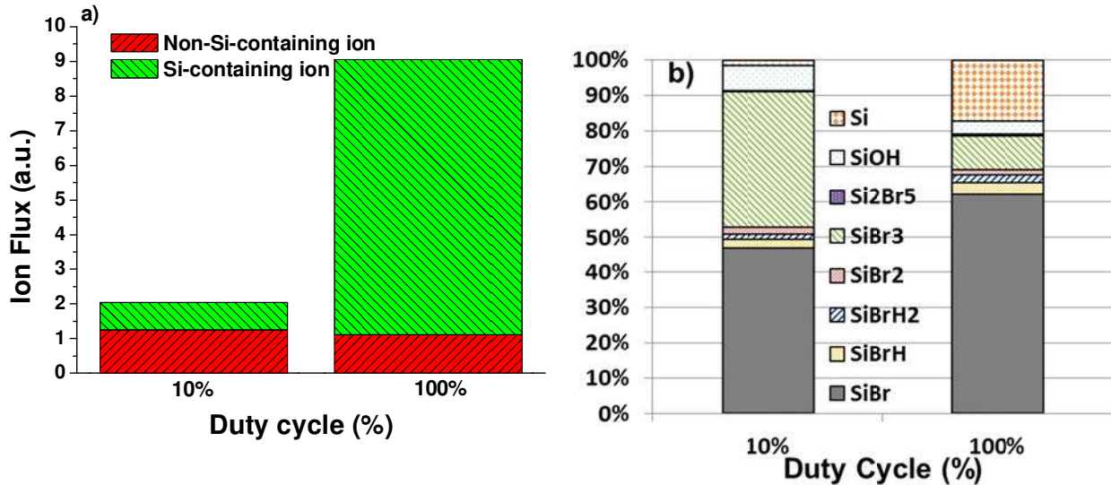
Figure 6. Ion flux composition during silicon etching in HBr/O 2 plasma pulsed at 1kHz. A duty cycle of 100% corresponds to the CW mode. a) Repartition between Si-containing ions and non-Si containing ions b) repartition of Si-containing ions
