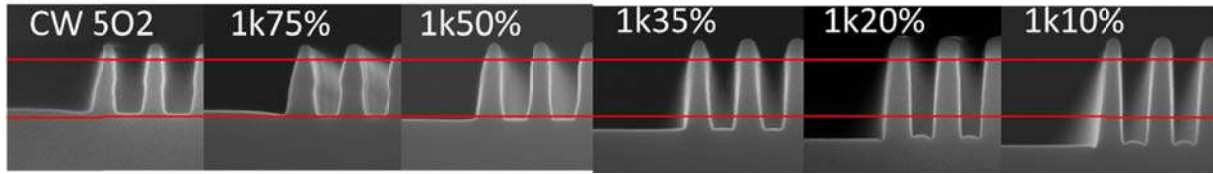
Figure 8. Semi isolated silicon patterns etched in an HBr/O 2 plasma pulsed 1 kHz and at various duty cycle with a SiO 2 hard mask. The etching time is set to have identical plasma ON time for all experiments (so-called time compensation)
