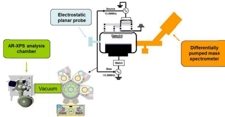
Figure 1. Schematic representation of the experimental setup, consisting in a pulsed ICP chamber equipped with differentially pumped mass spectrometry and an electrostatic planar probe. The chamber is connected under vacuum to an angle-resolved x-ray photoelectron spectroscopy system.
