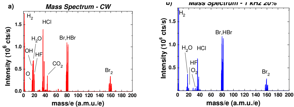
Figure 2. Mass spectra of neutral species present in the HBr/O 2 plasma at 0W bias power in a) continuous wave mode b) pulsed at 1kHz 20% DC
