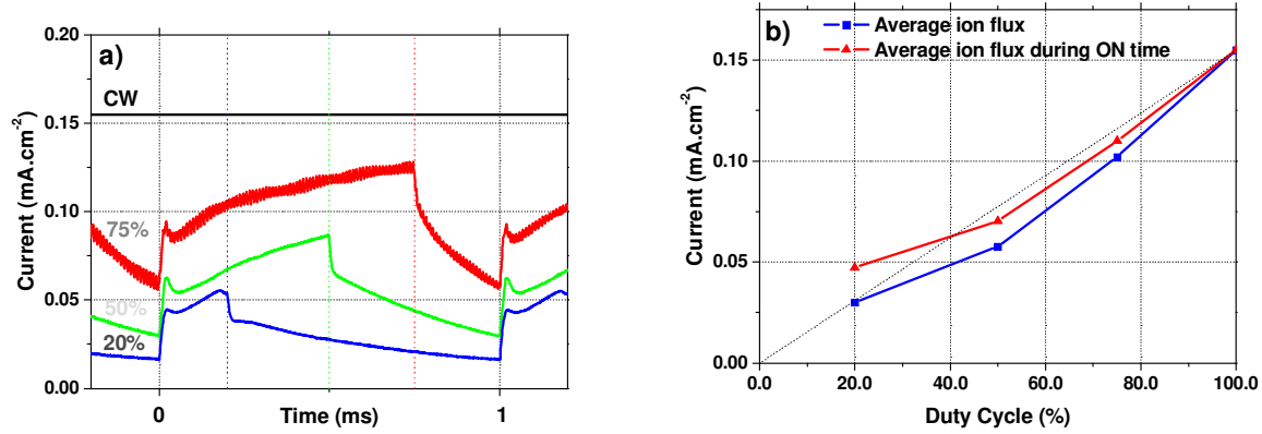
Figure 7. Ion flux measured during silicon etching in \text{HBr}/\text{O}_2 plasma pulsed at 1kHz. A duty cycle of 100% corresponds to the CW mode. a) time resolved measurement b) average ion flux and average ion flux during the plasma ON time only.
