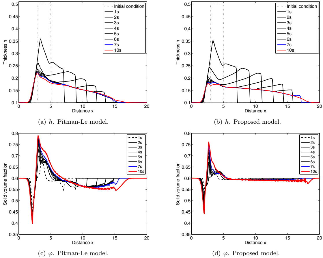
FIGURE 21. Test 2: The mass thickness h(x, t) in meters as a function of the distance x (m) (a-b) and of the solid volume fraction \varphi(x, t) as a function of the distance x (m) (c-d) at different times for the collapse of a rectangular granular mixture over an inclined layer ( \theta = 10^\circ ) made of the same mixture. The initial volume fraction is \varphi_0 = 0.6 . Here the friction law is the Richardson and Zaki drag force (RZ) with m = 1 .
