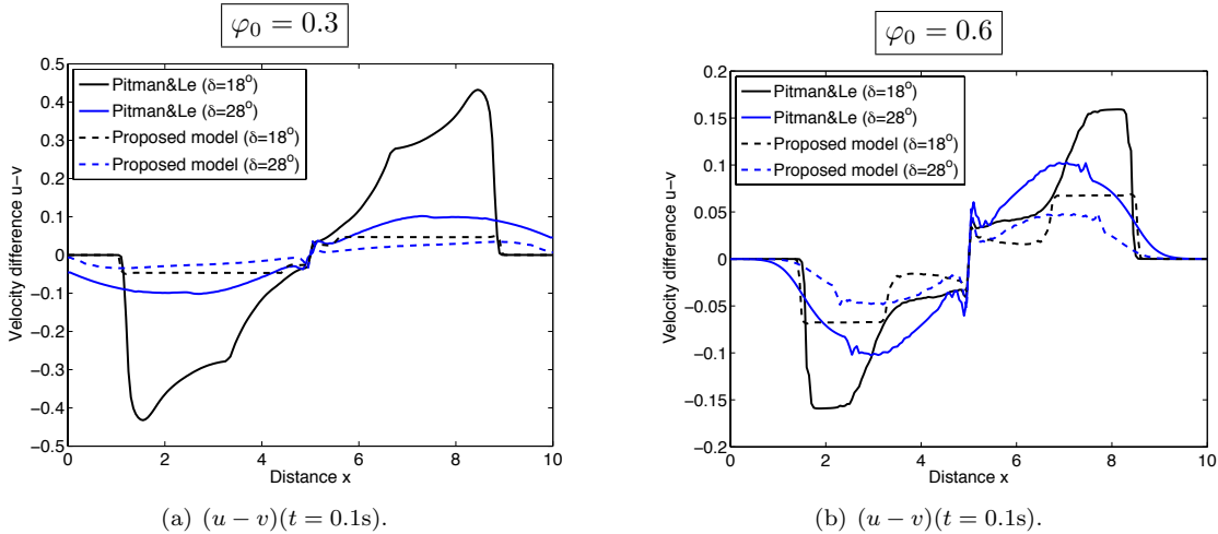
FIGURE 8. Test 1: Comparison of the difference of the fluid and solid velocities ( u - v ) ( \text{ms}^{-1} ) for the Pitman-Le and proposed models at time t = 0.1\text{s} for the collapse of a rectangular granular mixture over a horizontal layer made of the same mixture. The initial volume fractions are: (Left) \varphi_0 = 0.3 ; (Right) \varphi_0 = 0.6 . Here the friction law is the Richardson and Zaki drag force (RZ) with m = 1 .
