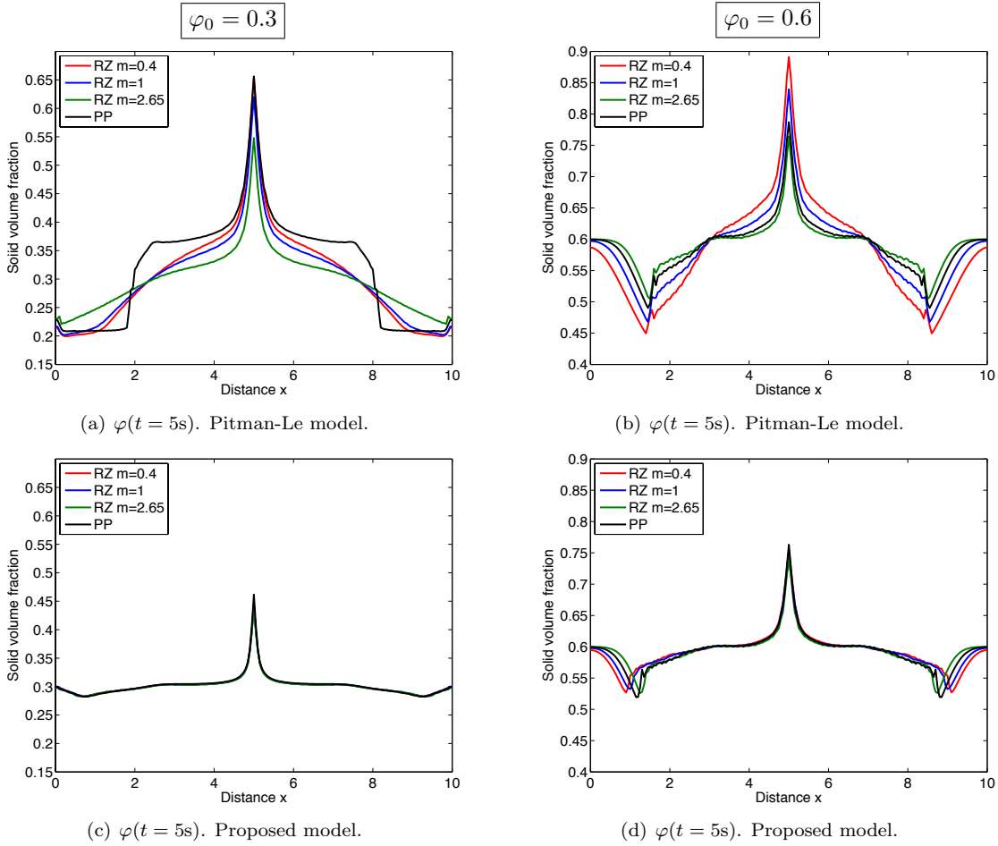
FIGURE 5. Test 1: Solid volume fraction of the mass \varphi as a function of the distance x (m) at time t = 5\text{s} , when the granular phase has already stopped, for the collapse of a rectangular granular mixture over a horizontal layer made of the same mixture, simulated with different friction laws (“RZ” refers to the Richardson and Zaki and “PP” to the Pailha and Pouliquen drag forces). The initial volume fractions are: (Left) \varphi_0 = 0.3 ; (Right) \varphi_0 = 0.6 .
