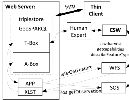
Fig. 2. Proposed architecture
