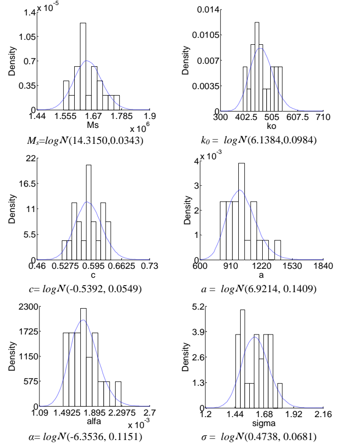
Figure 3: Histograms of parameters of M_1 model
