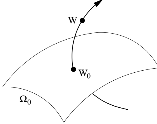
Figure 1. Fiber above the manifold of null velocity \Omega_0 . Thanks to the action of the group, a state W_0 of null velocity \Omega_0 generates a current state W .
