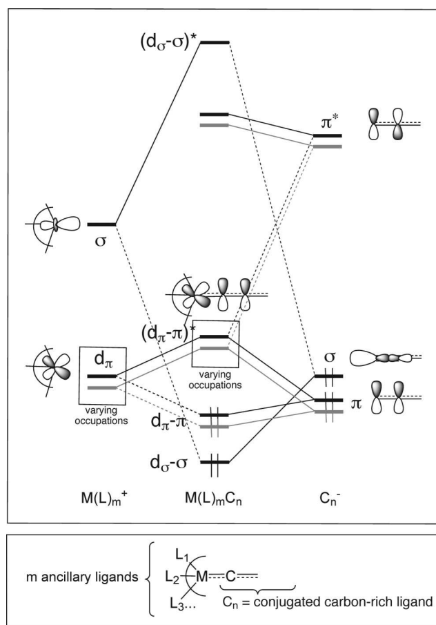
Scheme 3 Qualitative orbital interaction diagram between the frontier orbitals of a metallic fragment M(L_x)_m^+ and of a carbon-rich conjugated ligand C_n^- .
