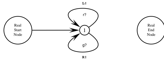
Figure 5: An ATN built by natural selection, implementing the best behavioral strategy.
