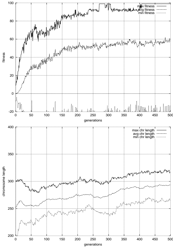
Figure 3: Evolution of the fitness and chromosome length (random insertions and deletions, r = 1\% , p = 20\% )
