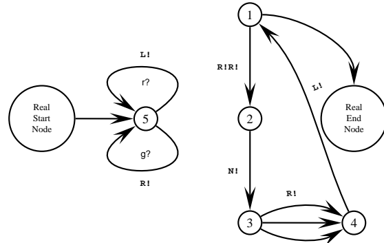
Figure 5: An ATN built by natural selection, implementing the best behavioral strategy.
