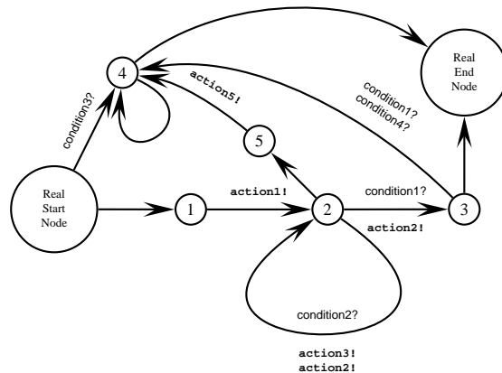
Figure 1: An example of ATN.
