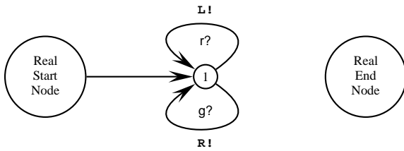
Figure 4: The “optimal” ATN (providing the highest fitness with the simplest structure).
