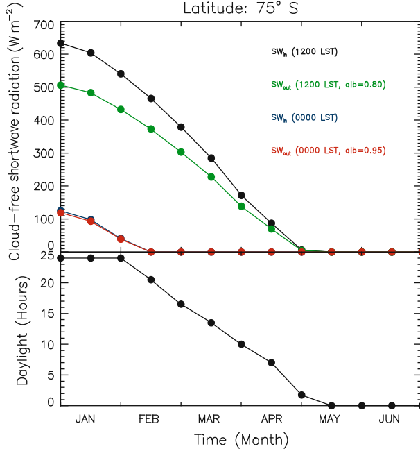
Fig. 2 Top Evolution from January to June for cloud-free conditions at 75°S and sea level of: incoming shortwave radiation at 1200 LST (black filled circles), and at 0000 LST (blue filled circles), outgoing shortwave radiation at 1200 LST with a surface albedo of 0.80 (green filled circles) and at 0000 LST with a surface albedo of 0.95 (red filled circles). Bottom daylight evolution at 75°S from January to June (Calculated from http://people.cas.sc.edu/carbone/modules/mods4car/shortwave/index.html ).
