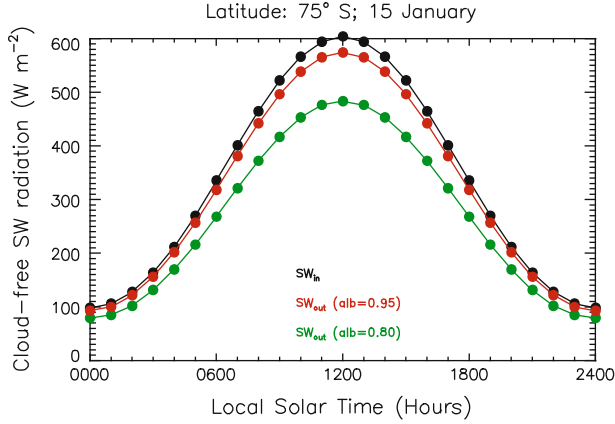
Fig. 1 Diurnal variation at 75°S on 15 January (LST) and at sea level for cloud-free conditions of: incoming shortwave radiation ( black filled circles ), outgoing shortwave radiation with a surface albedo of 0.95 ( red filled circles ) and a surface albedo of 0.80 ( green filled circles ) (Calculated from http://people.cas.sc.edu/carbone/modules/mods4car/shortwave/index.html .)
