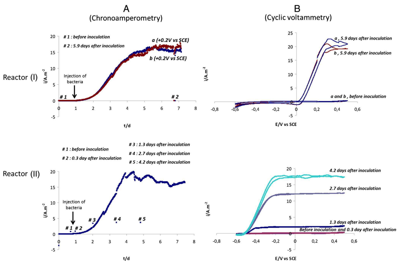
Fig. 1. Bioanodes formed with the original commercial G. sulfurreducens strain. A) Current density versus time (# indicate the interruptions for CV recording); B) Cyclic voltammeteries performed at 1 \text{ mV s}^{-1} during chronoamperometry. (I) Reactor with two electrodes polarized at +0.2 \text{ V/SCE} (a and b); CVs on electrodes a and b performed before bacteria injection and 5.9 days after bacteria injection. (II) Reactor with an electrode polarized at -0.2 \text{ V/SCE} ; CVs performed before bacteria injection, 0.3, 1.3, 2.7, and 4.2 days after bacteria injection.
