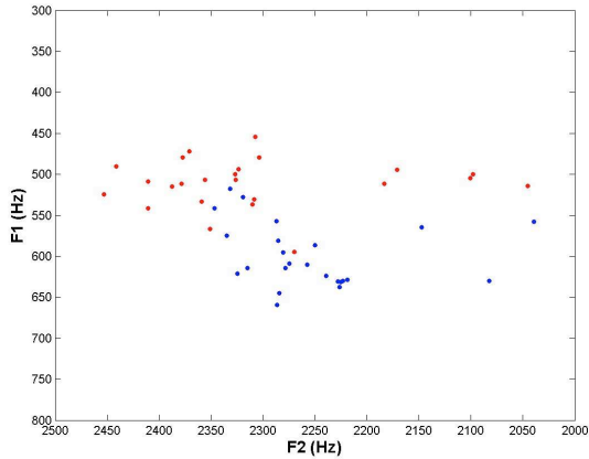
Figure 5: F1-F2 patterns for /ε/ as V_1 in all VCV sequences in the context of V_2 = /a/ (blue) and V_2 = /i/ (red), for an example adult speaker facing left.
