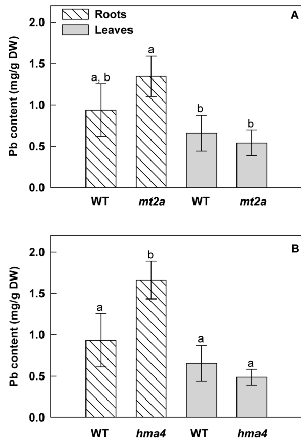
Figure 7. Lead accumulation in roots and shoots of wild-type and knockout mutant seedlings of A. thaliana . Seedlings were collected after 13 days of culture on agar plates with or without 40 μM of Pb(NO 3 ) 2 . (A) Atmt2a T-DNA mutant analysis. (B) Athma4 T-DNA mutant analysis. All results are the average value (± SE) of three independent replicates. For the roots and leaves separately, the letters represent statistically homogenous subgroups using LSD post hoc test at a \alpha=0.01 significance level. doi:10.1371/journal.pone.0061932.g007
