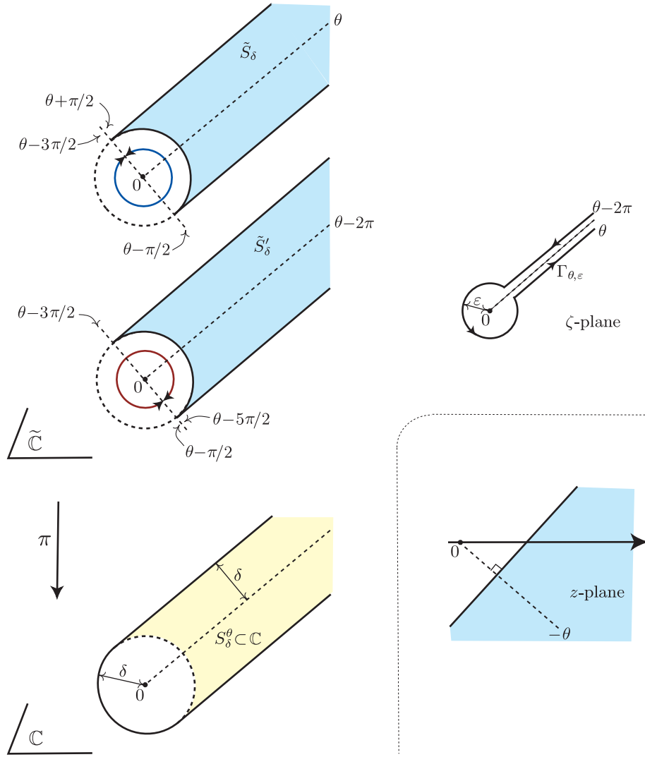
Figure 10: Laplace transform of a major . Left: the domain of \tilde{\mathbb{C}} where \check{\varphi} must be holomorphic and its projection S_\delta^\theta in \mathbb{C} . Right: the contour \Gamma_{\theta,\varepsilon} for \zeta (above) and the domain where z belongs (below).
