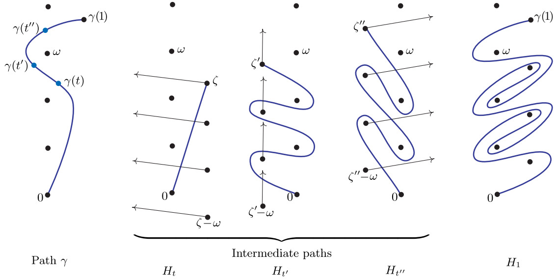
Figure 8: From \gamma to the integration path H_1 used for \text{cont}_\gamma(\hat{\varphi} * \hat{\psi})(\gamma(1)) .
