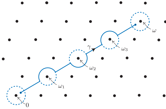
Figure 12: An example of path \gamma used in the definition of \mathcal{A}_{\omega,\varepsilon}^{\Omega} , here with \varepsilon = (-, +, -) .
