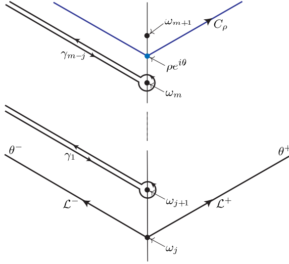
Figure 13: From the Stokes phenomenon to the symbolic Stokes automorphism.
