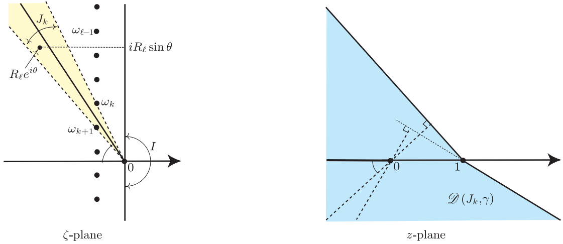
Figure 3: Borel-Laplace summation for Poincaré's example.
