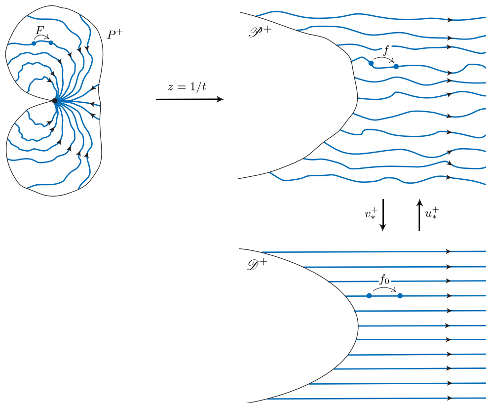
Figure 17: The dynamics in the attracting petal viewed in three coordinates.
