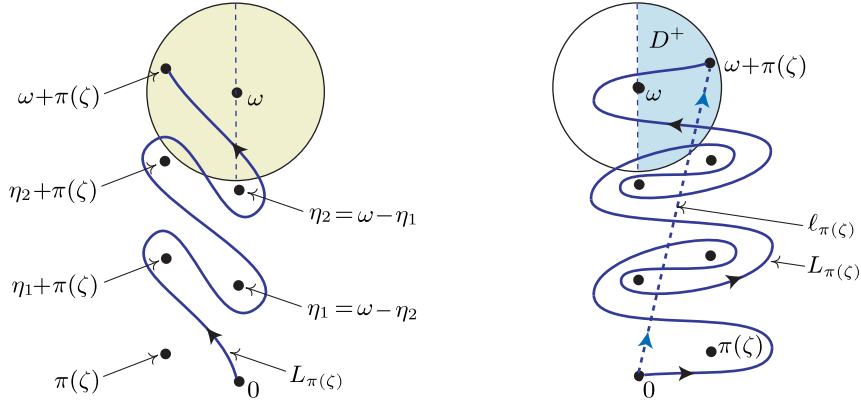
Figure 14: Integration paths for \hat{\varphi} * \hat{\psi} . Left: L_{\pi(\zeta)} for \arg \omega - 2\pi < \arg \zeta \leq \arg \omega - \pi . Right: \ell_{\pi(\zeta)} and L_{\pi(\zeta)} for \arg \omega - 3\pi < \arg \zeta \leq \arg \omega - 2\pi . (Case when \Sigma_\omega has two elements.)
