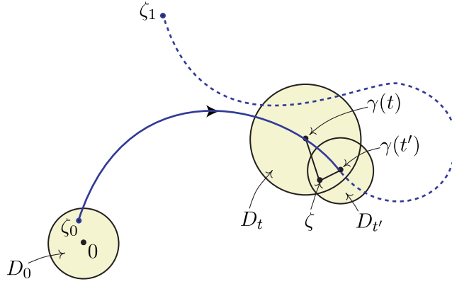
Figure 5: Integration paths for the convolution in the easy case.
