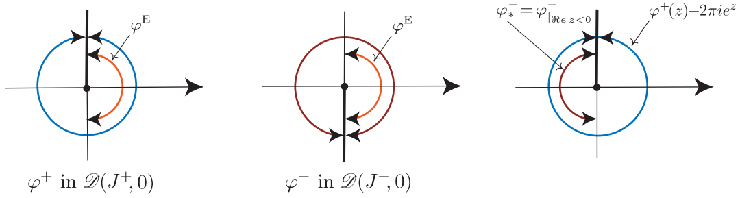
Figure 2: Borel sums of the Euler series. Left and middle: \varphi^\pm extends \varphi^E in the cut plane \mathcal{D}(J^\pm, 0) . Right: \varphi^+(z) - 2\pi i e^z extends \varphi_*^- = \varphi_*^-_{\{\Re z < 0\}} in the cut plane \mathcal{D}(J^+, 0) .
