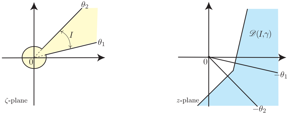
Figure 1: 1-summability in an arc of directions. Left: \hat{\varphi}(\zeta) \in \mathcal{N}(I, \gamma) is holomorphic in the union of a disc and a sector. Right: the domain \mathcal{D}(I, \gamma) where \mathcal{L}^I \hat{\varphi}(z) is holomorphic.
