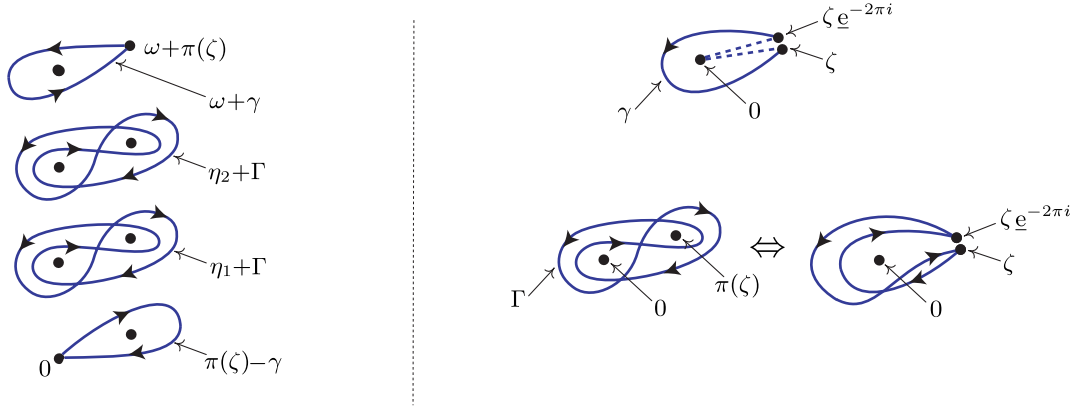
Figure 15: Computation of the variation of the singularity at \omega of \hat{\varphi} * \hat{\psi} .
