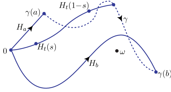
Figure 7: Symmetric \Omega -homotopy ( H_a = initial path, H_b = final path, \gamma = endpoint path \Gamma_H ).
