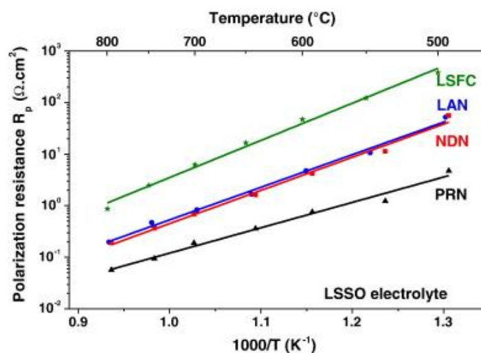
Fig. 11. Arrhenius plots of the polarization resistances for the electrode materials sintered on LSSO electrolyte at 1100 \text{ }^\circ\text{C} for 1 h.
