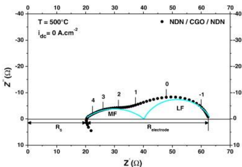
Fig. 8. Typical impedance diagram obtained at T = 500 °C, in air, for a symmetrical cell: NDN/CGO/NDN.
