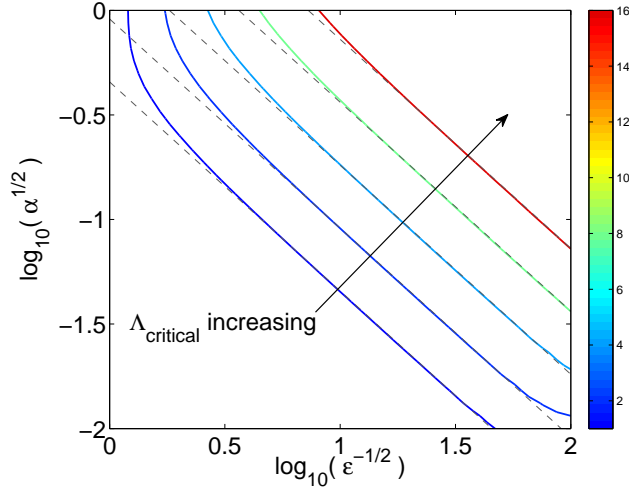
Fig. 5 Isovalue lines of \Lambda_{\text{critical}} = 1, 2, 4, 8, 16 (continuous line), compared to the approximated law (15) (dashed line). The approximated law fits well the isovalue lines for values of \alpha and 1/\varepsilon near to \alpha = 10^{-2} , \varepsilon = 10^{-2} . The map was obtained by a plot of isovalues of a matrix of 34 by 34 points.
