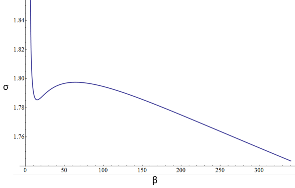
Figure 4. \beta vs \sigma for schedules satisfying the KKT conditions in a two job instance.
