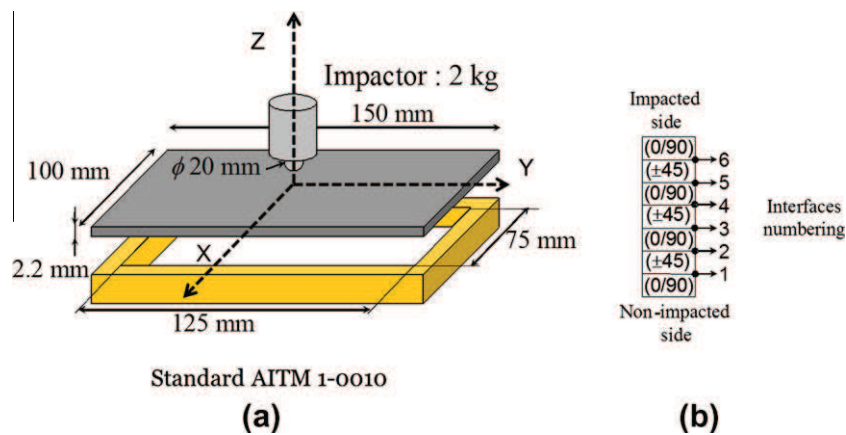
Fig. 1. Reference case: (a) impact set up, and (b) stacking sequence of the laminate.
