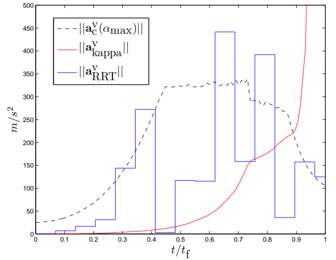
Fig. 9. Scenario 2 - Lateral accelerations along the solution trajectories
