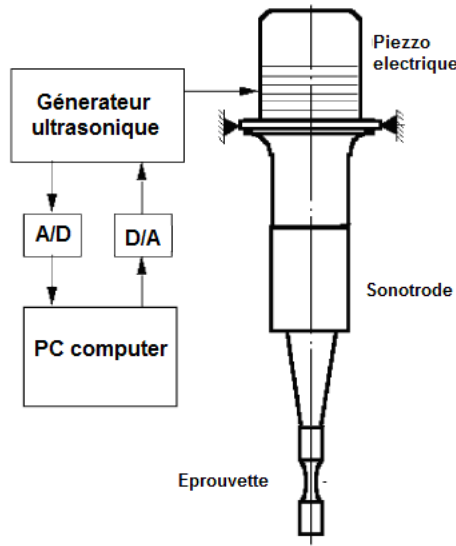
Figure 2. Scheme of the piezoelectric machine
