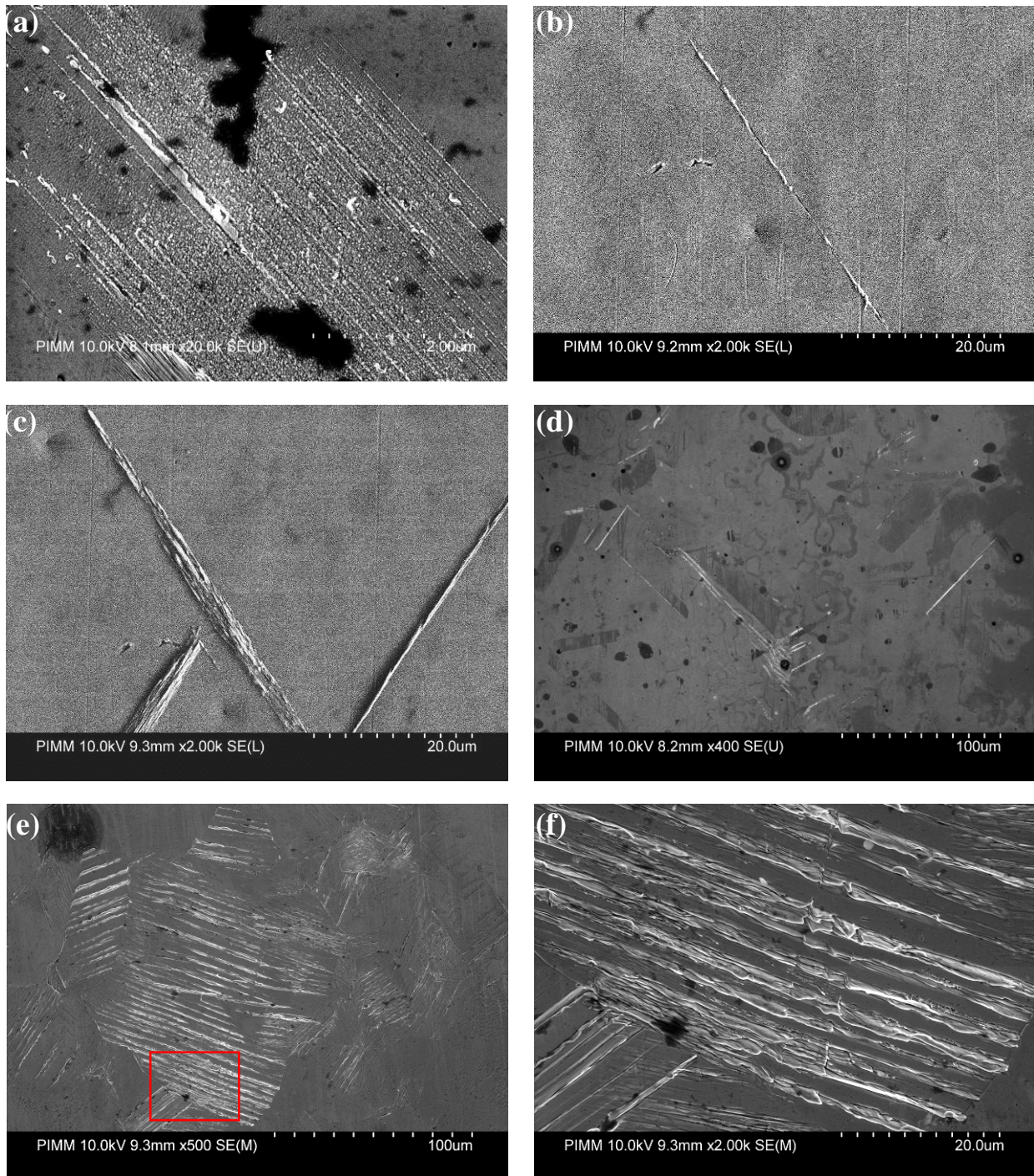
Figure 4. Scanning Electron Micrographs of the specimen surface - (a) \Delta\sigma/2 = 49.6 MPa - 10^8 cycles; (b) \Delta\sigma/2 = 54.7 MPa - 10^7 cycles and (c) at the same place after 10^8 cycles; (d) \Delta\sigma/2 = 69.4 MPa - 10^6 cycles; (e) \Delta\sigma/2 = 69.4 MPa - 10^7 cycles (f) zoom of (e)
