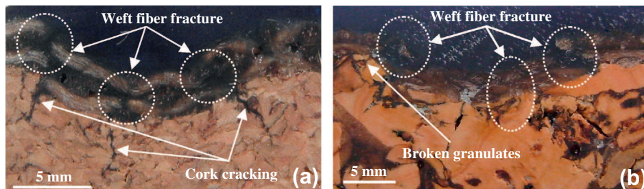
Fig. 12. Cross section photographs showing the damage state for two sandwich laminates with 7 J of impact energy. (a) SD 310 sandwich and (b) SD 160 sandwich.
