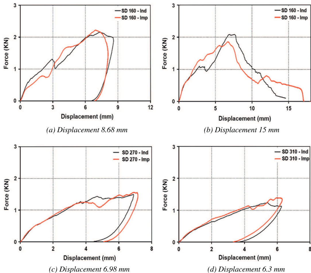
Fig. 13. Comparison of the force–indenter displacement curves for the indentation and impact tests on the jute/epoxy-cork sandwich laminates.
