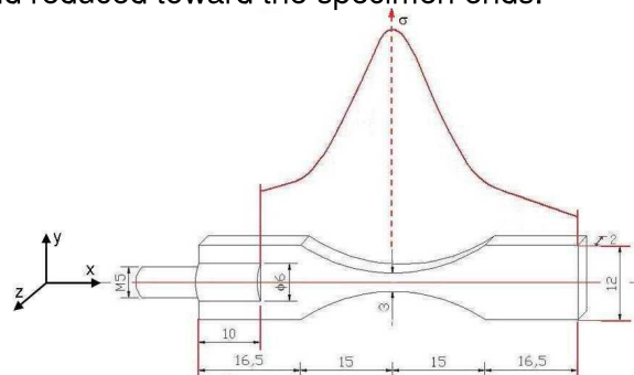
Fig 1 Ultrasonic fatigue plate specimen and distribution of stress along the specimen axis
