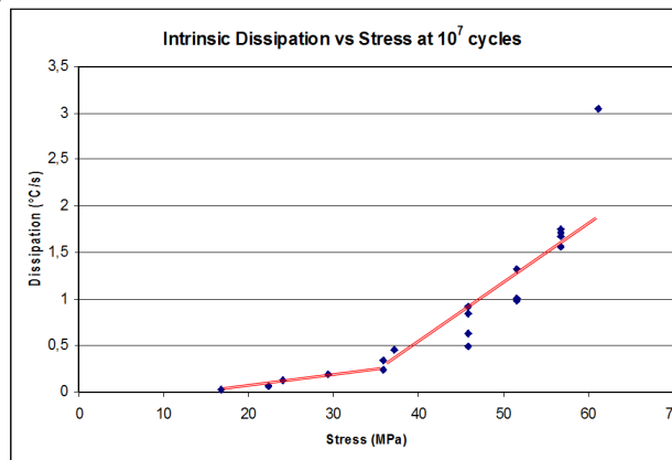
Fig 5. Average intrinsic dissipation at 10^7 cycles vs maximum stress amplitude
