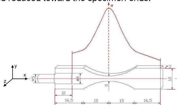
Fig 1 Ultrasonic fatigue plate specimen and distribution of stress along the specimen axis
