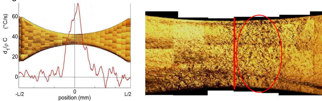
Fig 2. Intrinsic dissipation along the specimen at \Delta\sigma/2 = 72.1 MPa, 10^7 cycles and a zoom at the middle of specimen
