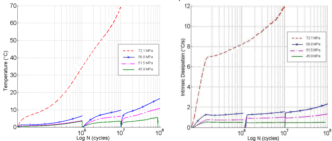
Fig 3. (a) Average temperature and (b) Average intrinsic dissipation during fatigue test at different constant stress amplitude fatigue test.
