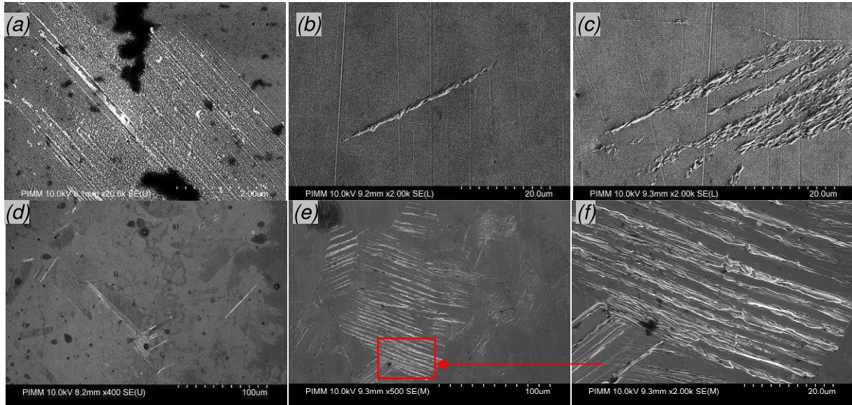
Fig 4. SEM micrographs of specimen surface at (a) \Delta\sigma/2 = 51.5 MPa after 10^8 ; at \Delta\sigma/2 = 56.8 MPa (b) after 10^7 cycles and (c) the same position after 10^8 cycles; at (d) \Delta\sigma/2 = 72.1 MPa after 10^6 cycles (e) \Delta\sigma/2 = 72.1 MPa after 10^7 cycles (f) a magnification of (e)
