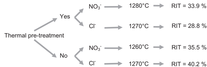
(c) 200ppm La_2O_3 -doping – RIT Measurement ( \lambda = 640 nm – th. = 0.88mm)
