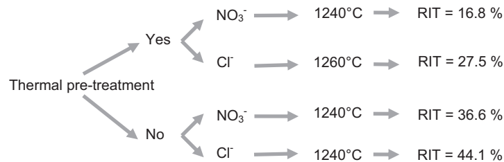
(b) 200ppm ZrO_2 -doping – RIT Measurement ( \lambda = 640 nm – th. = 0.88mm)
