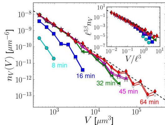
FIG. 5. Domain volume distribution n_v(V) (except percolating domain) after thermal treatment at T=1130 °C during 8, 16, 32, 45 and 64 min. The dotted line is n_V \sim V^{-\beta} , with \beta = 1.7 . The open symbols show the size distributions before the correction due to the finite size of the field of view. The inset shows the same results after rescaling by the dynamical length \ell(t) .
