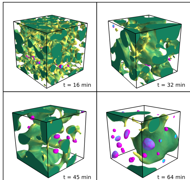
FIG. 1. 3D visualization[34] of the barium-rich phase, from scans after different times at 1130 °C (16, 32, 45 and 64 min). The color codes represent the absolute value of the mean curvature: shades of green for the percolating domain, shades of purple for isolated domains. The lateral size of the cube is 140 \mu\text{m} . The coarsening of the structure is accompanied by a fragmentation of the spanning cluster into isolated domains.
