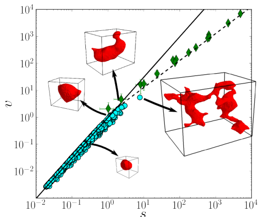
FIG. 3. Rescaled volumes v of the domains vs their rescaled surfaces s , for all isolated domains (cyan circles) and for the percolating domain (green diamonds) after 16, 32, 45 and 64 min at 1130 °C. The error bars indicate the standard deviation of the measures for all boxes of a given size. The black solid line is v = s^{3/2} (ideal spheres), and the black dotted line is v \sim s . Some domains shapes are shown as examples.
