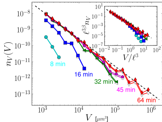
FIG. 5. Domain volume distribution n_V(V) (except percolating domain) after thermal treatment at T=1130 celsius during 8, 16, 32, 45 and 64 mn. The dotted line is n_V \sim V^{-\beta} , with \beta = 1.7 . The open symbols show the size distributions before the correction due to the finite size of the field of view. The inset shows the same results after rescaling by the dynamical length \ell(t) .
