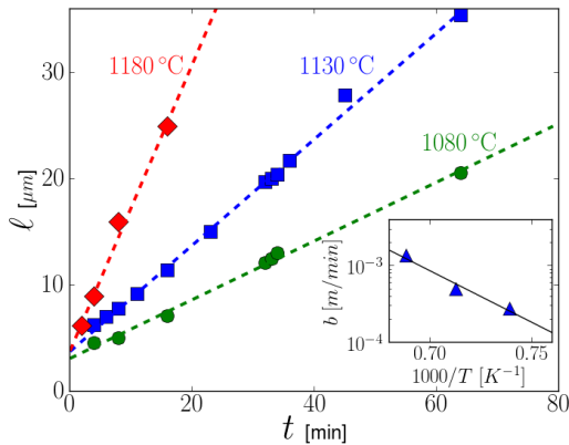
FIG. 2. Characteristic length \ell vs time t , for temperatures: 1080 °C (green circles), 1130 °C (blue squares), 1180 °C (red diamonds). The dotted lines are linear fits. Inset: semi-log plot of the slopes of the linear fits b , as a function of the inverse temperature 1/T .
