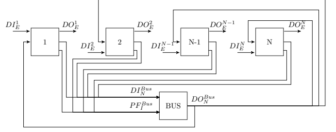
Fig. 6. Connected mode automata that model a fieldbus any moment one and only one terminal sends data to the bus (correct operation of the bus controller) will be made:
