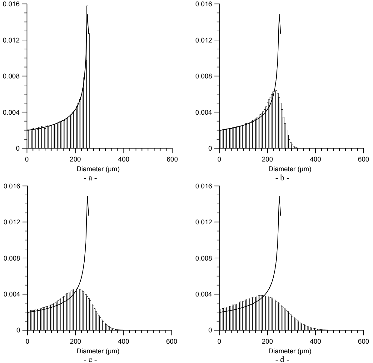
Figure 2. Grain-size histograms (6 \mu\text{m} -width class) in the DDRX model for pure nickel at 900 ^{\circ}\text{C} strained at 0.1 \text{ s}^{-1} – M coefficient of variation: 0 (a), 10 % (b), 20 % (c), 30 % (d) – Continuous line is the analytical solution for fixed M value as in the (a) case, final drop is due to the partial last class (252–258 \mu\text{m} , maximal diameter about 255.5 \mu\text{m} )
