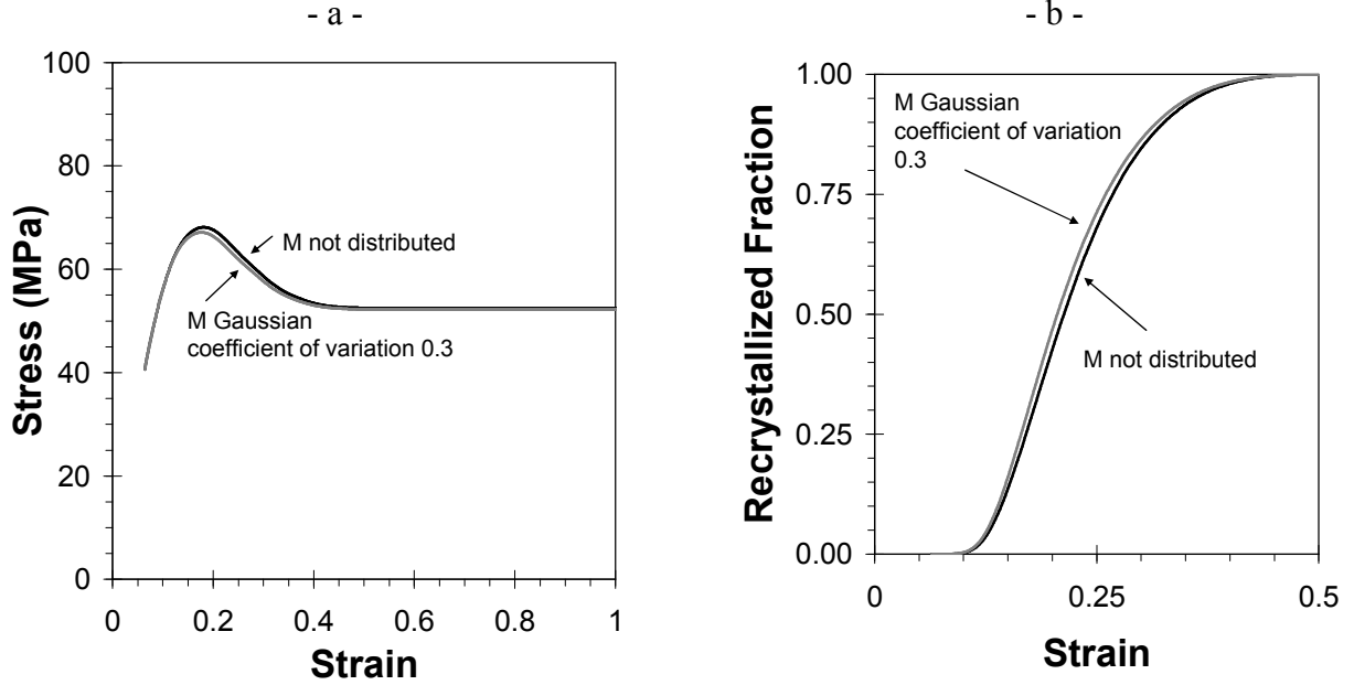
Figure 3. Comparisons between not distributed and Gaussian distributed grain-boundary mobility in terms of flow stress (a) and recrystallized fraction (b)
