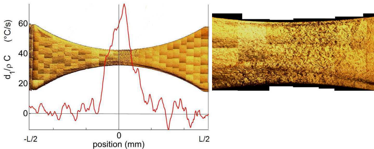
(a) (b) Figure 5. Intrinsic dissipation along the specimen at \Delta\sigma/2 = 72.1 MPa, 10^7 cycles (a) and a zoom at the middle of gauge specimen (b)
