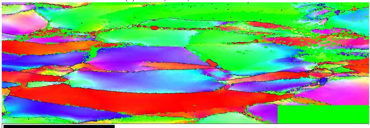
(a) 915 °C, \varepsilon = 1 , \dot{\varepsilon} = 0.01 \text{ s}^{-1}
