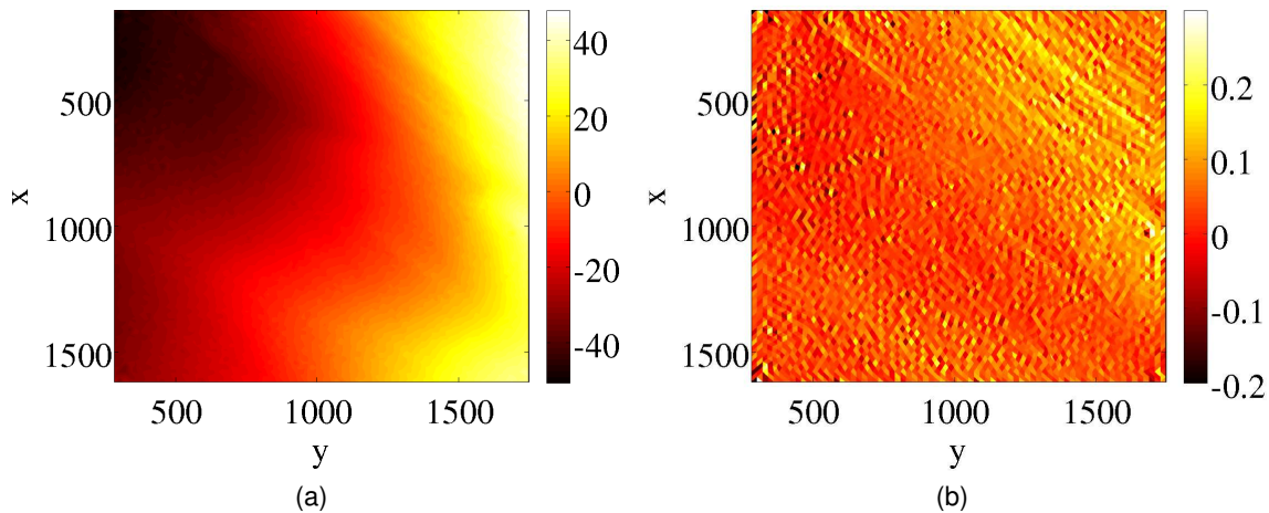
Figure 3 - Longitudinal displacement field in pixels (a) and longitudinal strain field (b) measured for macroscopic strain of 5%. The physical size of one pixel is 0.26 \mu m
