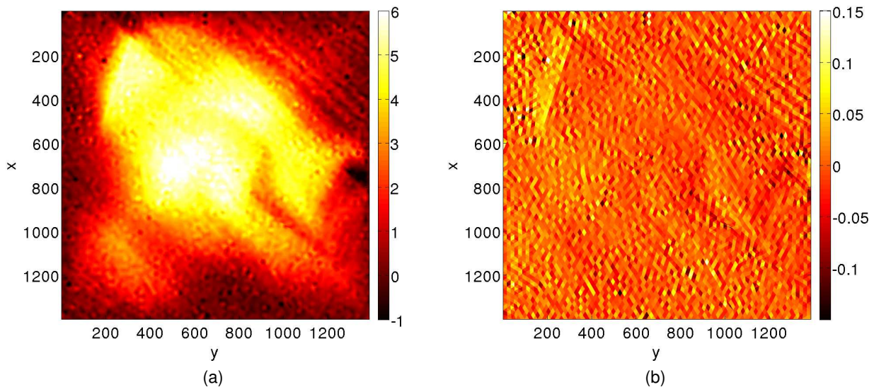
Figure 4 - Difference between fields measured by DIC and fields simulated by finite element with an initial value of the parameters, of longitudinal displacement in pixels (a) and longitudinal strain (b), for a macroscopic applied strain of 3%
