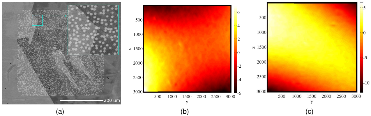
Figure 2 - Backscattered Electron (BSE) image of the deposited speckle (a). Displacement field in pixels along the x -direction (b) and the y -direction (c) resulting from both lithography and SEM imaging. The physical size of one pixel is 0.13 \mu m
