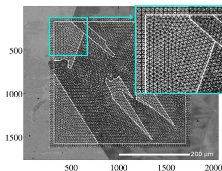
Figure 1 - Unstructured mesh compatible with the underlying microstructure for DIC analyses of the tensile test
