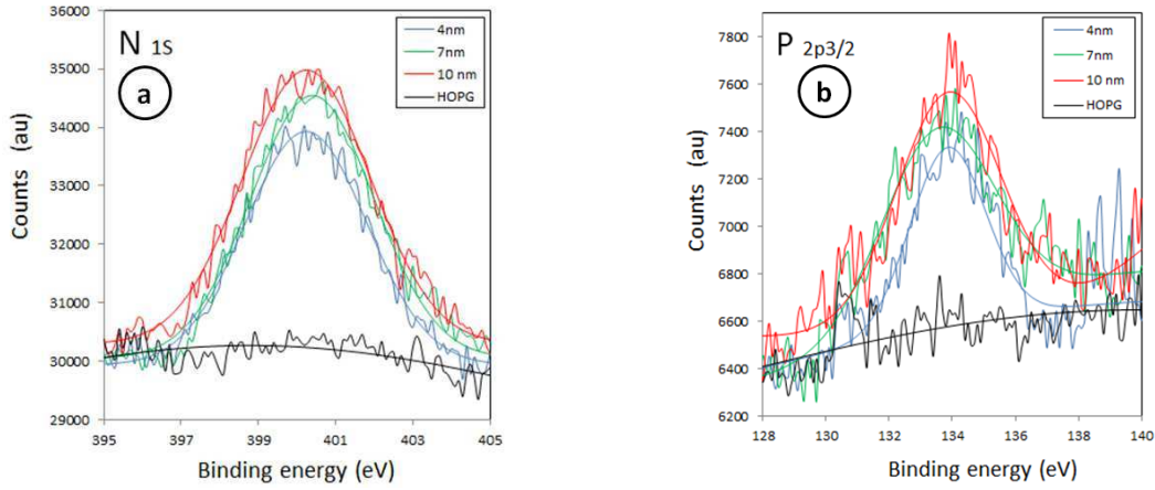
Figure 6: (a) N 1s and (b) P 2p3/2 XPS spectra of the three layers of DNA-Dap 2+ and of the pristine HOPG substrate in the same binding energy region. The blue, green and red lines correspond respectively to the fittings realized using the XPS peak fitting program on the 4, 7 and 10 nm thick layers.
