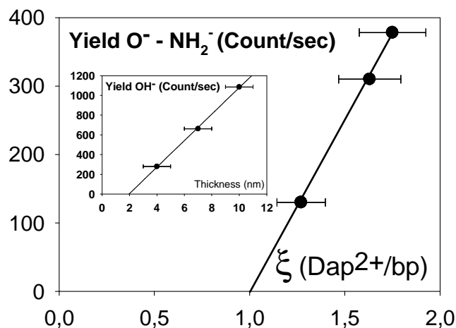
Figure 7: Yields O - - NH 2 - versus \xi , number of Dap 2+ per base pair in the films. Inset, OH - yields as a function of the thickness of the same films. The error bars represent statistical deviations (see the text for more details). The lines are linear regressions with R^2 = 0.9991 and 0.9993 respectively.
