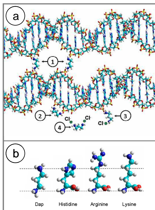
Figure 1: (a) Schematic view of the specific sites where Dap^{2+} cations interact with the DNA phosphate moieties. (1) correspond to the linking of two double-strands belonging or not to a same plasmid DNA, (2) corresponds to the electrostatic binding of a Dap^{2+} cation to two consecutive anionic phosphate moieties along the DNA's backbone (the special case where Dap^{2+} is capable of pronounced narrowing of the minor groove through direct binding to the phosphate groups across the groove 30 is not shown here for clarity). (3) illustrates the case where one Dap^{2+} cationic site remains free, (4) shows the Dap^{2+} diamine where both ammonium sites are counterbalanced with chloride anions in solution. (b) Size and structure comparison of the Dap molecule with the three basic amino acids histidine, arginine and lysine that interact with the DNA phosphate moieties in histones in the cellular environment. (b) are HyperChem(TM) snapshots of molecular mechanics optimizations based on the Block-diagonal (Newton-Raphson) method.
