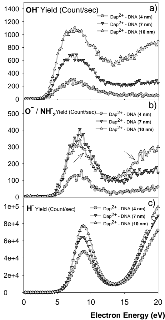
Figure 4: The yield functions of (a) OH^- , (b) O^- / NH_2^- and (c) H^- obtained from three DNA- Dap^{2+} films with 4, 7 and 10 nm thicknesses and from a clean HOPG surface. In panel (b), two arrows indicate the special behaviour of the yield function observed when comparing the 7 nm to the 10 nm layer, where an inversion of the yields occurs from the resonance region (DEA) compared to the monotonically increasing region of DD. The lines through the data points serve only as a guide to the eye.
