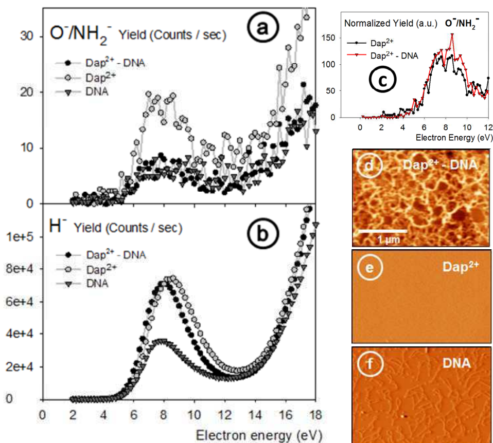
Figure. 3 (a) and (b): Incident electron energy dependence of respectively O^-/NH_2^- and H^- yields from thin films of: 1,3-diaminopropane( Dap^{2+} ), supercoiled plasmid DNA and DNA- Dap^{2+} complexes deposited on HOPG. (c) Normalized yields of O^-/NH_2^- signals for the Dap^{2+} and Dap^{2+} - DNA layers. (d), (e) and (f) AFM ( 3 \times 2 \mu m ) tapping mode images of the corresponding samples; they were all recorded with the same magnification (see d for the scale). The AFM images show (d) a Dap^{2+} -DNA thin film of 4 nm thickness, (e) the surface of a Dap^{2+} deposit, where the molecules are not visible on the image owing to the limited spatial (lateral) resolution of the AFM in air, and (f) Individual DNA plasmids spread on the HOPG surface.
