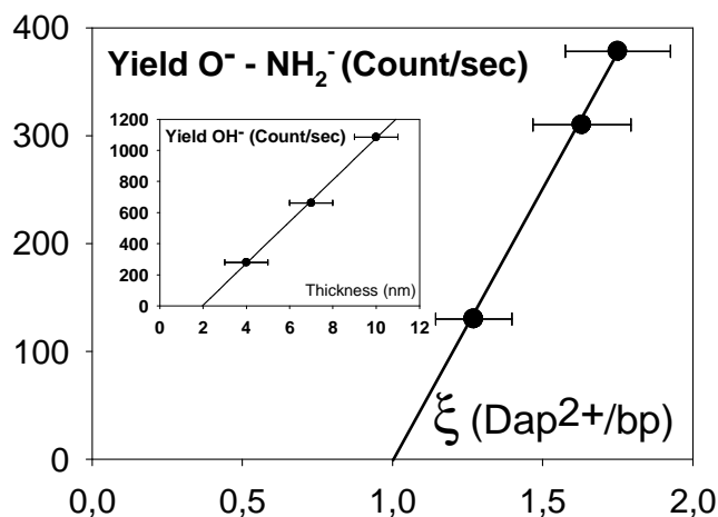
Figure 7: Yields O^- - NH_2^- versus \xi , number of Dap^{2+} per base pair in the films. Inset, OH^- yields as a function of the thickness of the same films. The error bars represent statistical deviations (see the text for more details). The lines are linear regressions with R^2 = 0.9991 and 0.9993 respectively.
