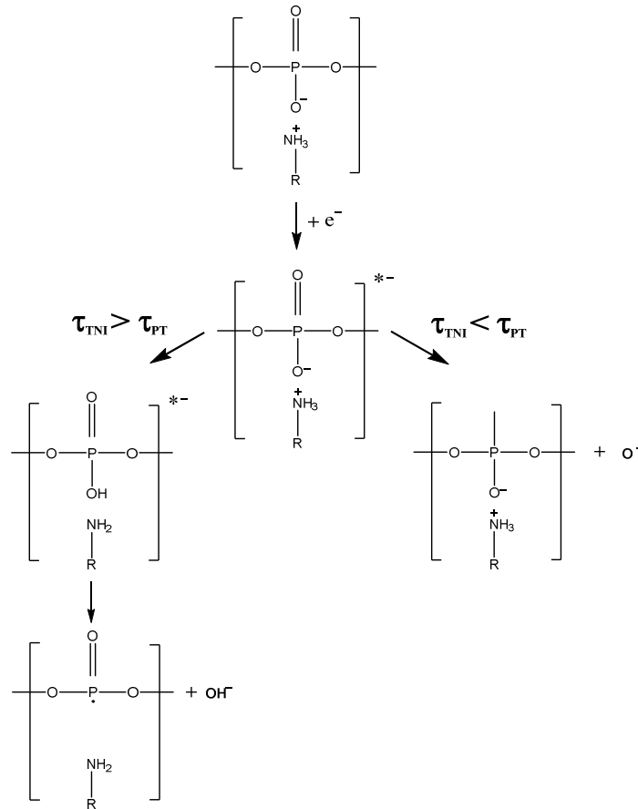
Figure 5: The two possible dissociative channels of the Transient Negative Ion (TNI) where the charged products are either \text{OH}^- or \text{O}^- , depending on the proton transfer mean lifetime ( \tau_{\text{PT}} ) as compared to the TNI lifetime ( \tau_{\text{TNI}} ).
