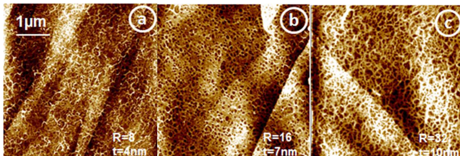
Figure 2: AFM tapping mode images of DNA-Dap films constructed on HOPG with molar ratios R = [\text{Dap}^{2+}]/[\text{PO}_4^-]_{\text{DNA}} = 8, 16 and 32 , respectively for (a), (b) and (c), prepared with C_{\text{DNA}} = 20 \text{ ng}/\mu\text{L} . In such conditions, the films have respectively thicknesses of 4, 7 and 10 nm.
