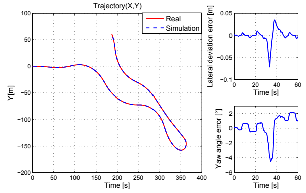
Fig. 5. Trajectories: Real (reference) and simulation (control law)
