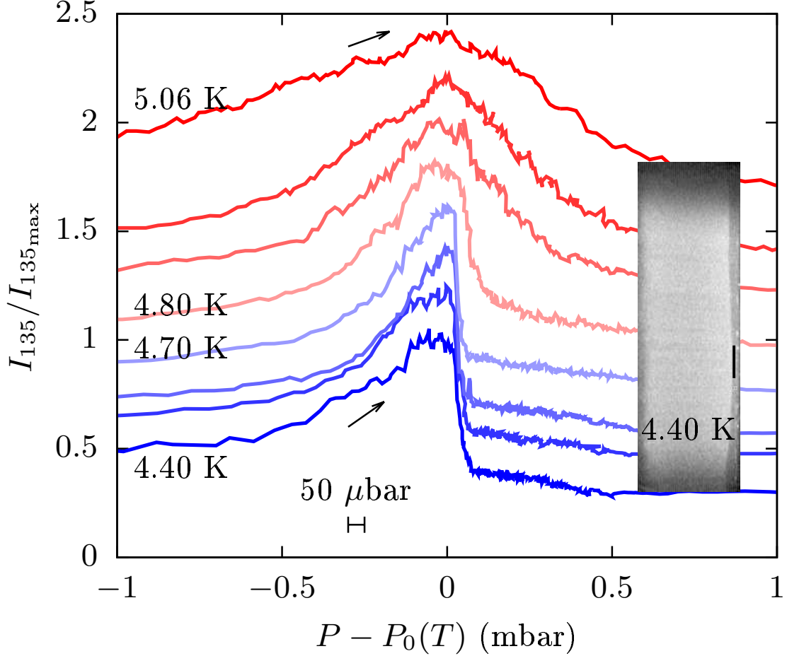
FIG. 3. (color online) Intensity scattered at 135^\circ (from the region marked by a black rectangle on the inset picture) during condensation at the temperatures of Fig. 1(b). P_0(T) is the pressure at which the optical signal is maximum at a given temperature. The y scale applies to the 4.40 K curve, the other curves are vertically shifted by 0.2 for clarity.
