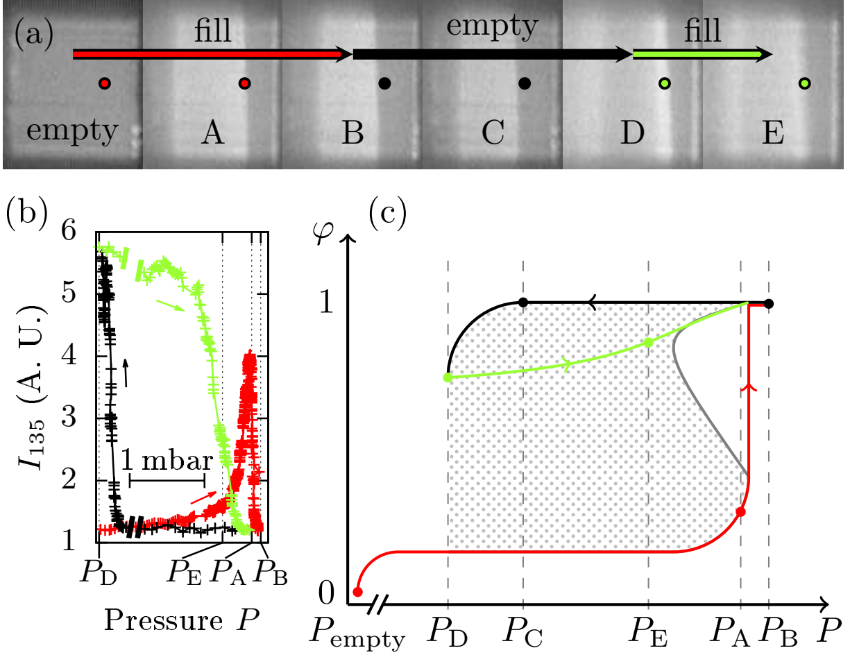
FIG. 4. (color online) (a) Central parts of pictures taken along a minor hysteresis loop at T = 4.6 K ( < T^* ). (b) Corresponding optical signal from the dot in Fig. 4(a) as a function of pressure. In chronological order, dark grey/red : initial filling; black: partial emptying; light grey/green: filling from the partially emptied state. (c) Hypothetical distribution of metastable states (shaded area, only shown for P > P_D ) in the (P, \varphi) plane, and paths deduced from the local optical signal in Figs. 4(a) and (b).
