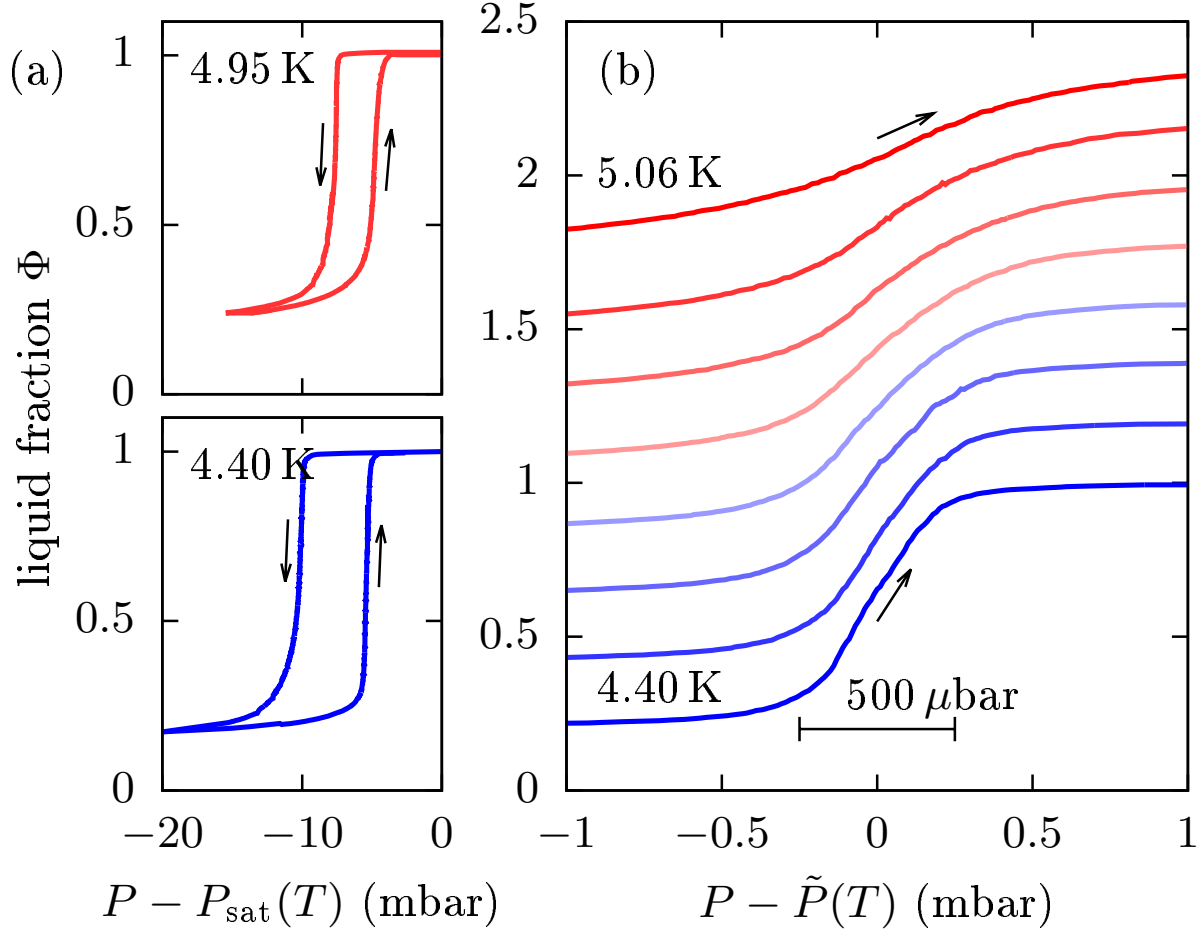
FIG. 1. (color online) (a) Hysteresis between adsorption and desorption isotherms at T = 4.40 K and 4.95 K. P_{\text{sat}}(T) is the bulk vapor pressure. (b) Adsorption isotherms for T = 4.40 K, 4.50 K, 4.60 K, 4.70 K, 4.80 K, 4.90 K, 4.95 K and 5.06 K. \tilde{P}(T) is the pressure at which the slope of the isotherm is maximum. The y scale applies to the 4.40 K curve, the other curves are vertically shifted by 0.2 for clarity.
