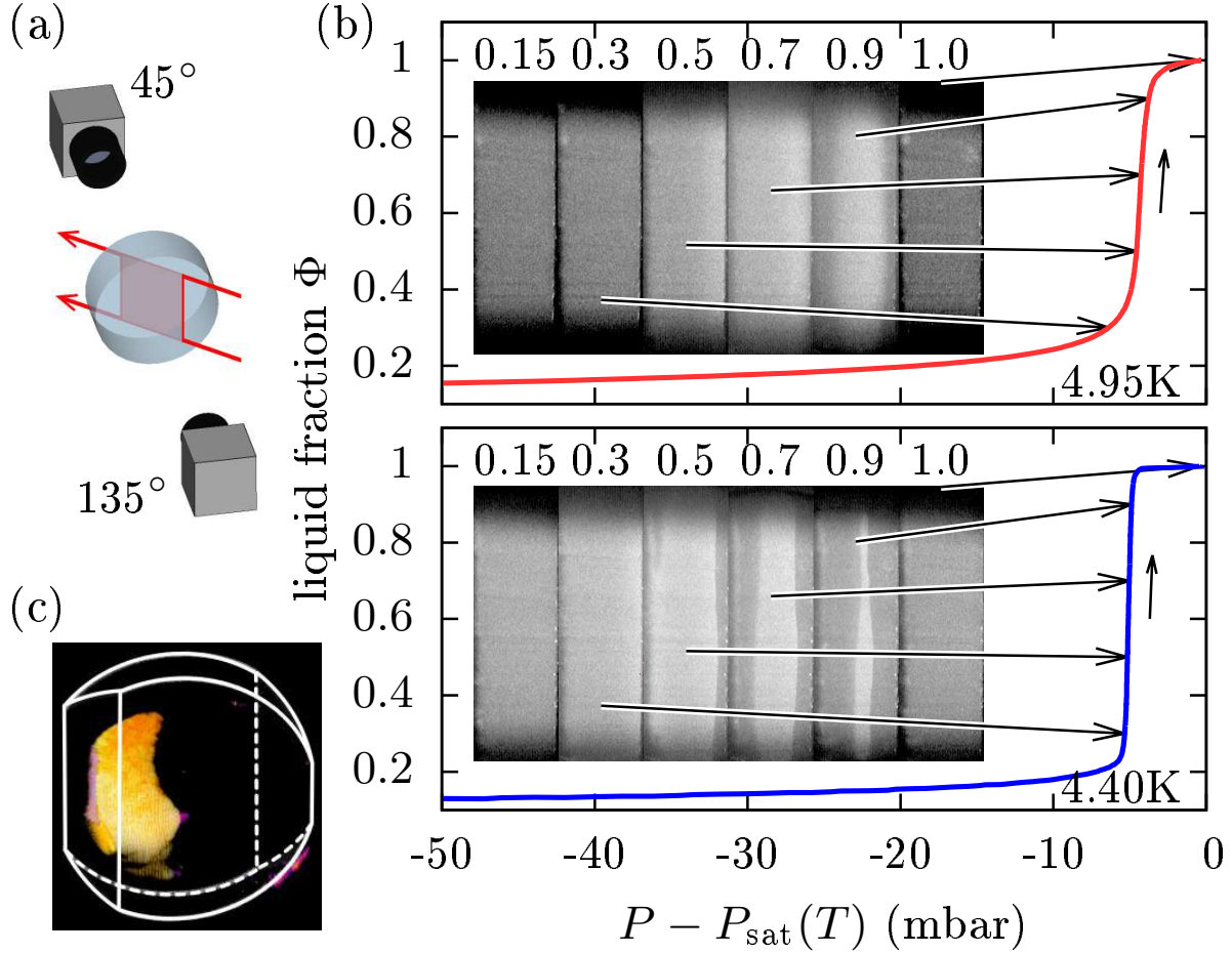
FIG. 2. (color online) (a) Positions of the laser sheet and of the CCD cameras relative to the aerogel. (b) Pictures of the illuminated region (1 cm height) taken with the 135° CCD (logarithmic grayscale) at increasing liquid fractions (given above the pictures) during isotherms at T = 4.40 K and 4.95 K. The arrows show the corresponding points on the isotherms. (c) Perspective view of a 3D tomographic reconstruction (see text) close to the end of the condensation isotherm ( \Phi \approx 0.95 ) at 4.60 K. The bright region, i.e. the not yet filled part of the aerogel, is located in its left part.
