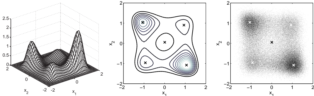
Figure 3: 2D problem (47)-(55). Left picture: 3D plot of the Gibbs density (38). Middle picture: ten level curves of the Gibbs density are represented in solid lines (the five extrema are represented with crosses). Right picture: a numerical trajectory \{X_n\} of the scheme (57) (with h = 0.02 , T = 2 \cdot 10^3 ).
