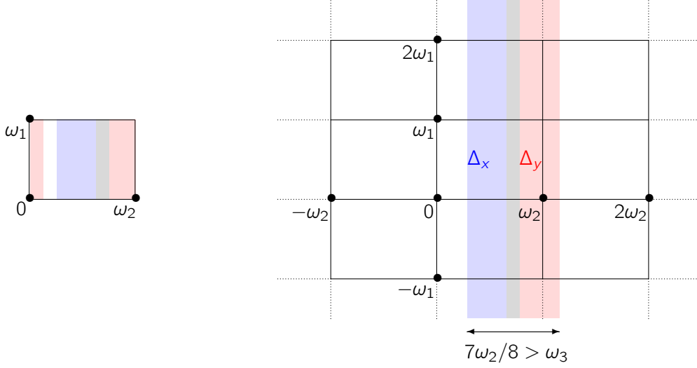
Figure 2. Left: the subdomains of the fundamental parallelogram [0, \omega_1] + [0, \omega_2] where |x(\omega)| < 1 (blue), |y(\omega)| < 1 (red) and |x(\omega)|, |y(\omega)| < 1 (grey). Right: corresponding domains \Delta_x (blue) and \Delta_y (red) on the universal covering \mathbf{C}_\omega . The intersection \Delta_x \cap \Delta_y is represented in grey. The domain \Delta = \Delta_x \cup \Delta_y has length 7\omega_2/8 , which is larger than \omega_3 = 3\omega_2/4 .
