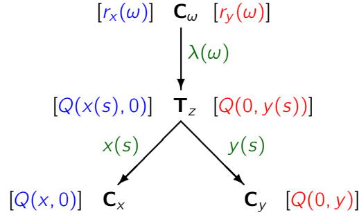
Figure 3. The GF Q(x, 0) is defined on (a subdomain of) the complex plane \mathbf{C}_x . It will be lifted on the Riemann surface \mathbf{T} as s \mapsto Q(x(s), 0) , and on the universal covering \mathbf{C}_w as r_x(w) = K(x(w), 0)Q(x(w), 0) . The same holds for Q(0, y) . We have also represented the projections between the different levels.
