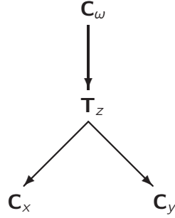
Figure 2. Different levels in our proof
